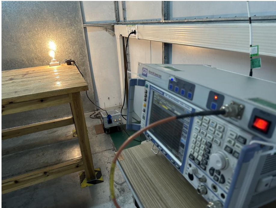
Test Setup For Conducted Emission
