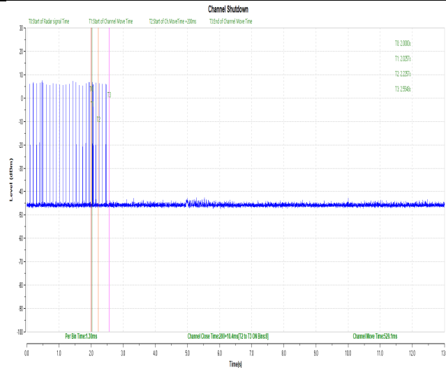
11A-5260-Type0-PASS
