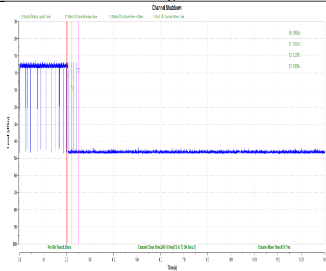
11A-5500-Type0-PASS
