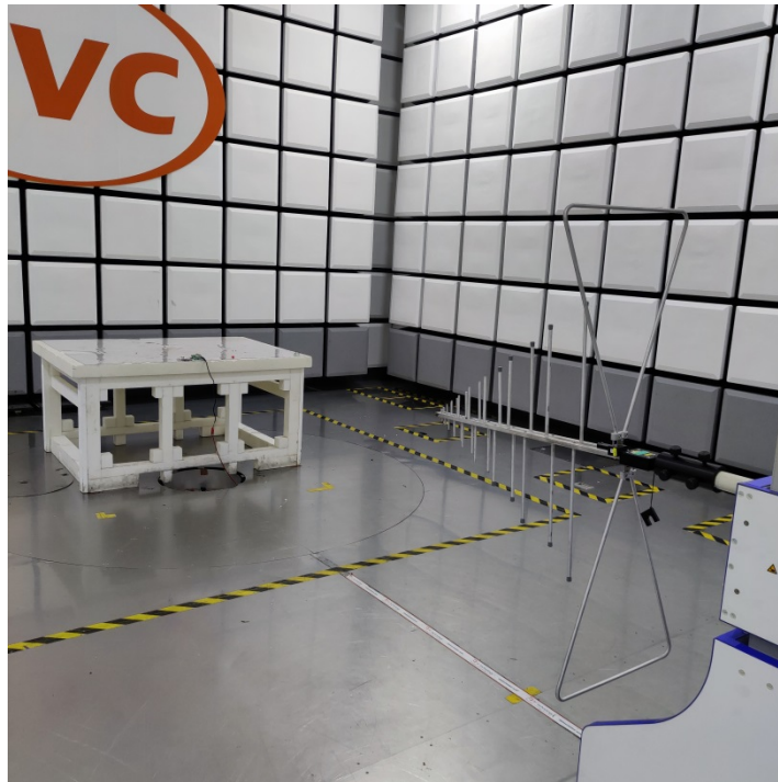
(2) Radiated spurious emission Test Setup(Below 1GHz)
