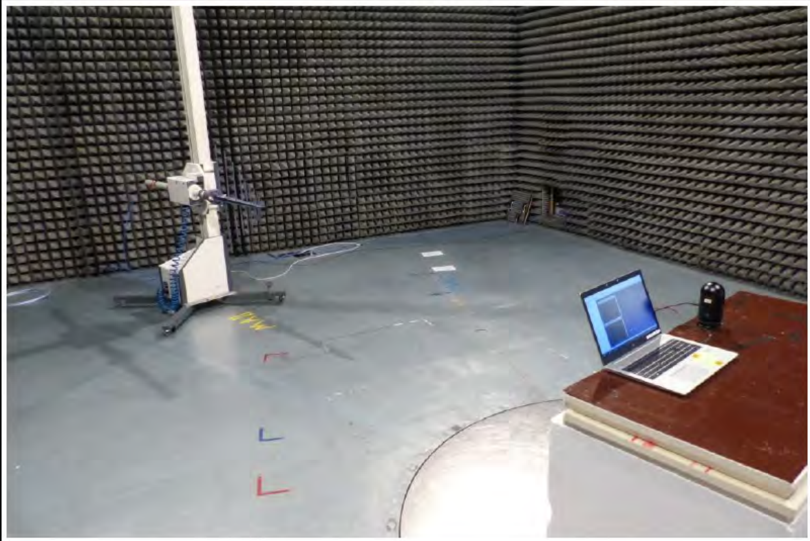
Test setup EUT Configuration II: 200-1000MHz
