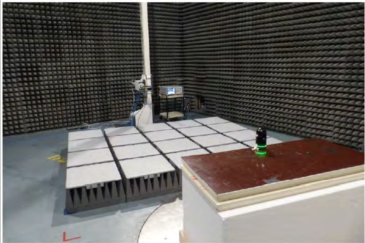
Test setup EUT Configuration I: 26500-30000MHz
