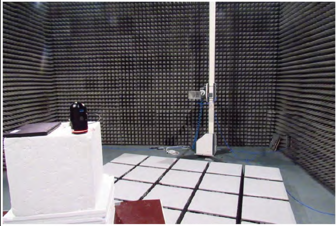
Setup 1-6.5 GHz
