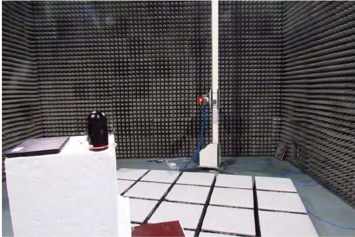
Setup 18-26 GHz
