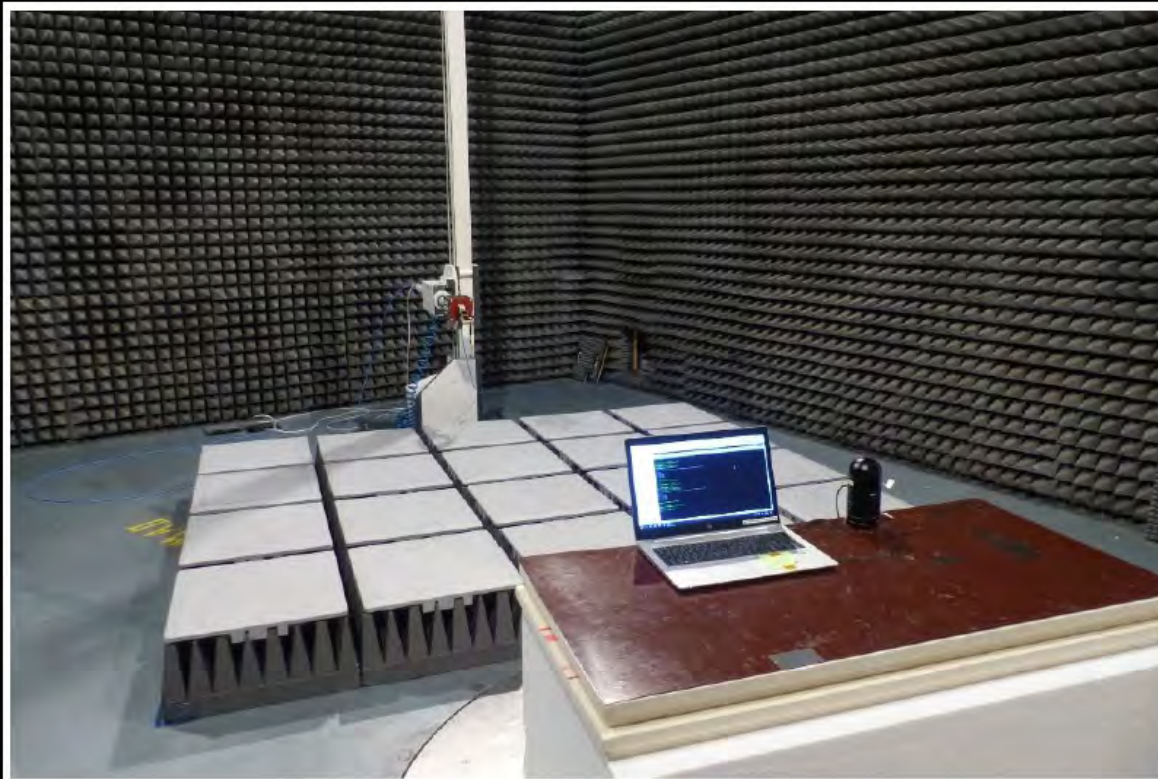
Test setup EUT Configuration II: 17000-26500MHz
