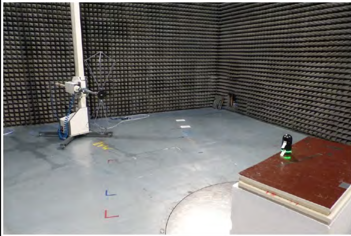
Test setup EUT Configuration I: 30-200MHz
