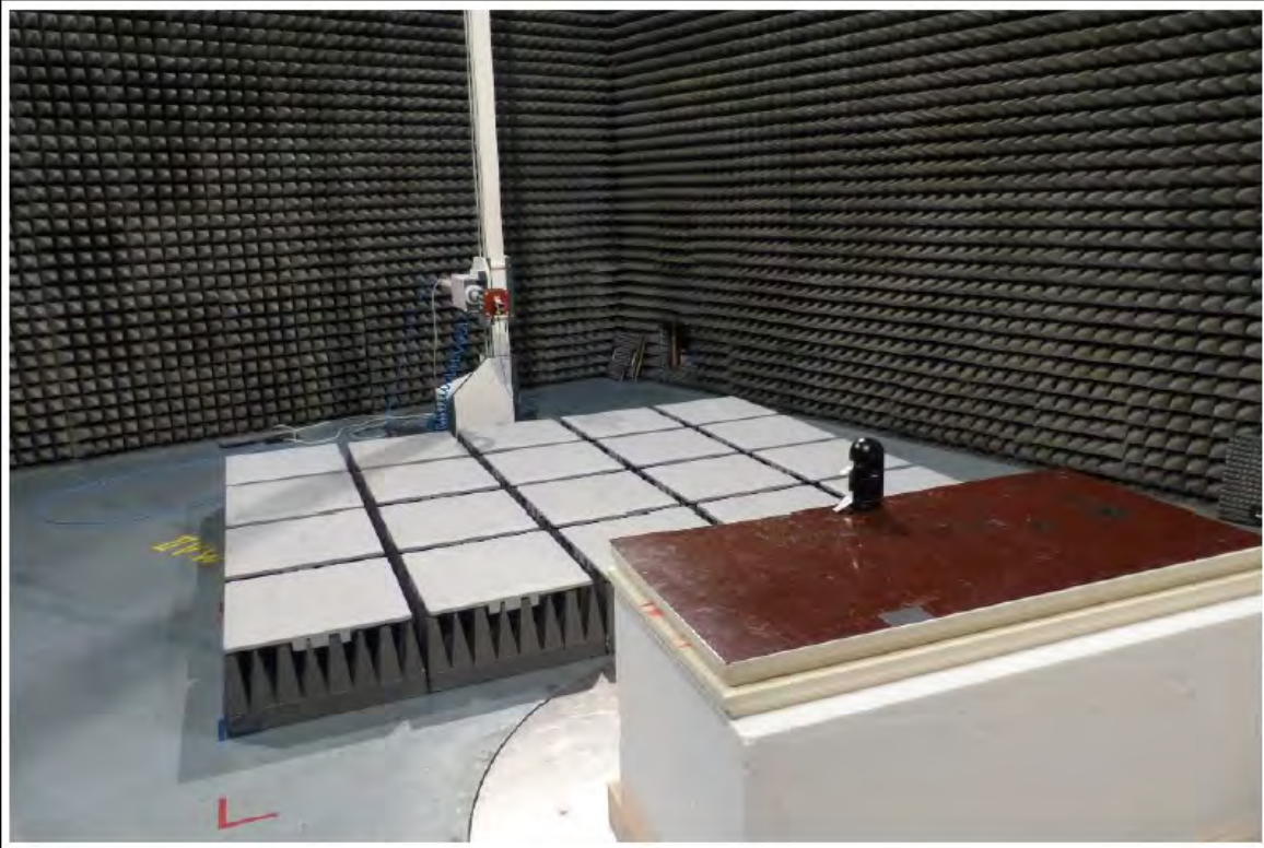
Test setup EUT Configuration I: 17000-26500MHz
