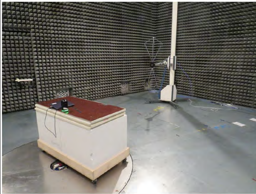
Setup 30 - 200 MHz
