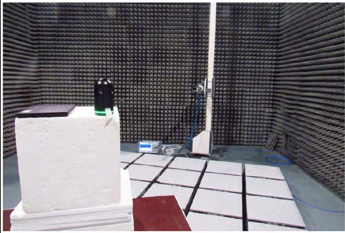
Setup 26 - 40 GHz
