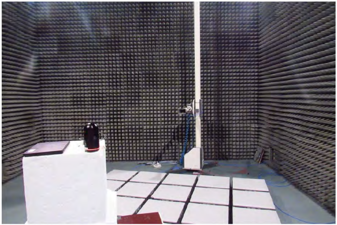
Setup 6.5-18 GHz
