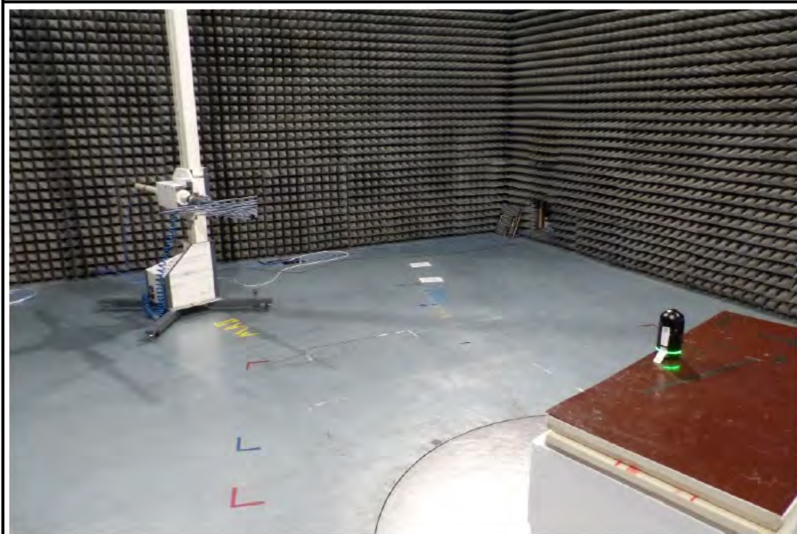
Test setup EUT Configuration I: 200-1000MHz
