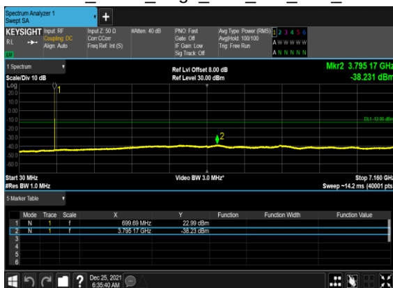
B2_N12(10M)_DFT-s- OFDM_BPSK_Edge_1RB_Left_Low_CH
