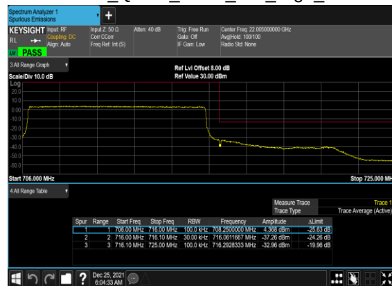
B2_N12(10M)_DFT-s- OFDM_QPSK_Outer_Full_High_CH
