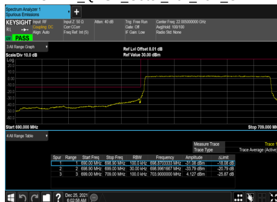
B2_N12(10M)_DFT-s-OFDM_QPSK_Outer_Full_Low_CH
