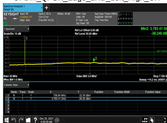
B2_N12(10M)_DFT-s- OFDM_QPSK_Edge_1RB_Left_High_CH
