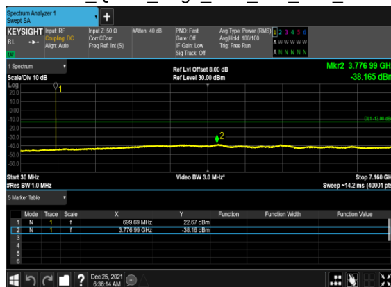
B2_N12(10M)_DFT-s- OFDM_QPSK_Edge_1RB_Left_Low_CH
