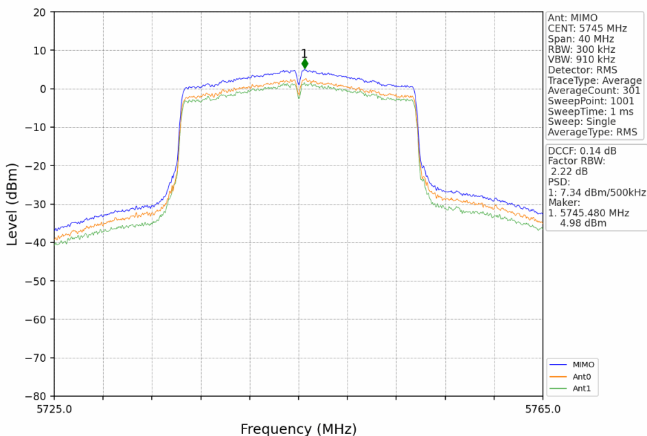
802.11ax(HEW20)_LCH_5745MHz_RU242_Left_MIMO_NTNV
