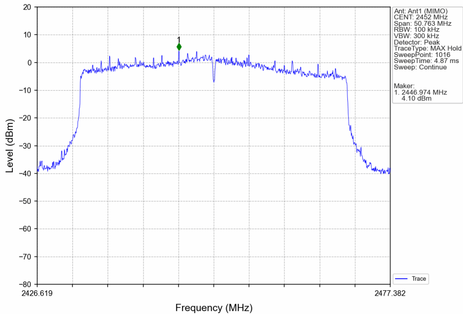
802.11ax(HEW40)_HCH_2452MHz_SU_/_Ant1 (MIMO)_NTNV
