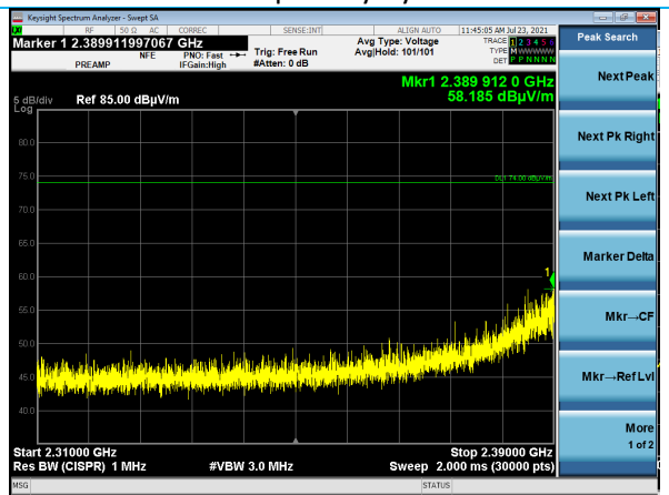
2310-2390 MHz, Peak 802.11n MCS0, Channel 1
