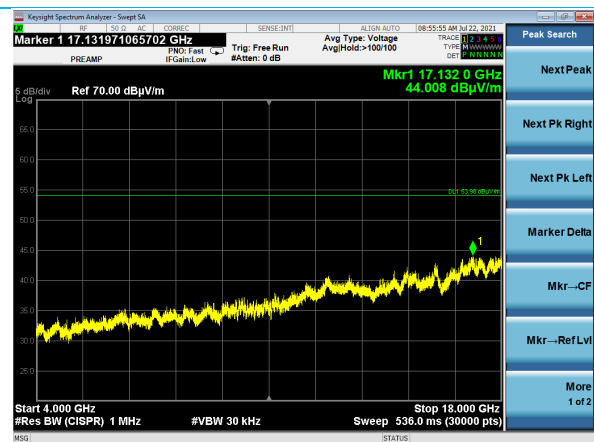
4-18 GHz, Vertical Antenna 802.11b 1Mbps, Channel 11
