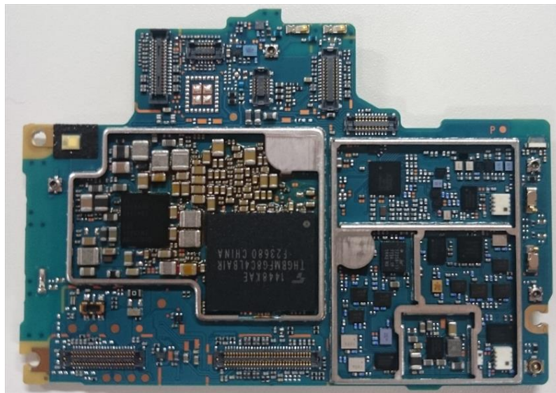
Internal PWB without Shield cases (Rear-side)
