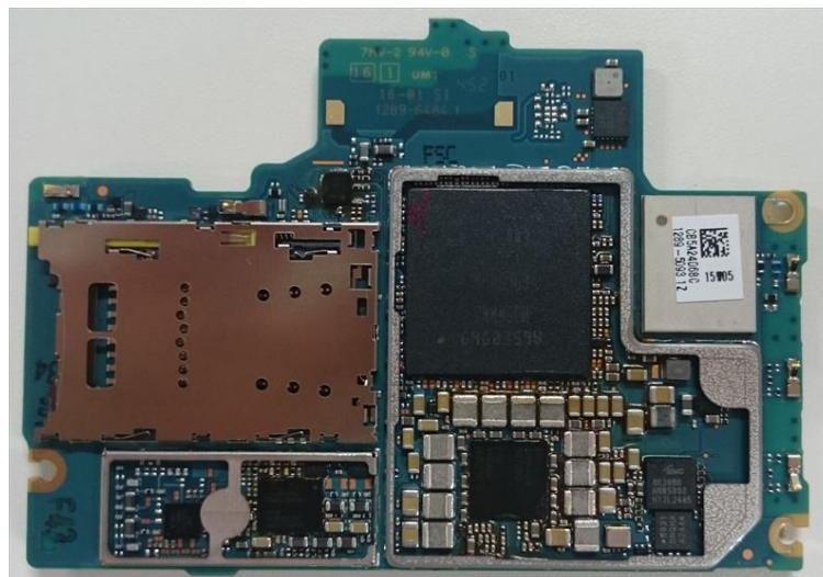
Internal PWB without Shield cases (Front-side)
