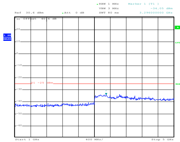
Figure 8.2-2: UL 406.125 MHz Spurious 1-5 GHz
