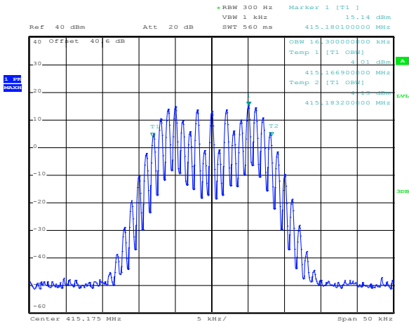
Figure 8.4-10: UL analog input Plus 3 dB
