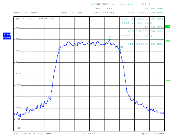
Figure 8.4-6: UL P25 input Plus 3 dB
