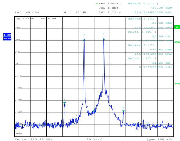
Figure 8.2-8: Intermodulation f_0 - UL 3.125 kHz, f_0 + 3.125 kHz Plus 3 dB
