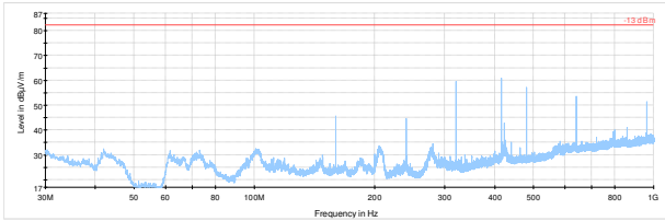
Figure 8.3-1: 30-1000 MHz UL
