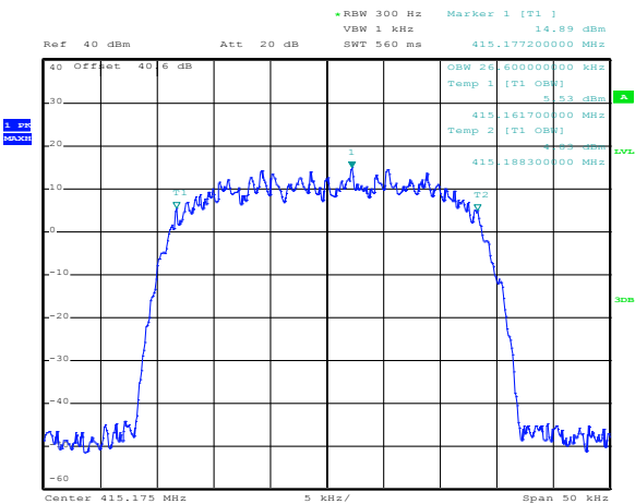
Figure 8.4-2: UL TETRA input Plus 3 dB
