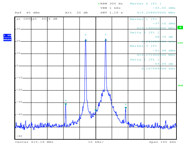
Figure 8.2-7: Intermodulation f_0 - UL 3.125 kHz, f_0 + 3.125 kHz
