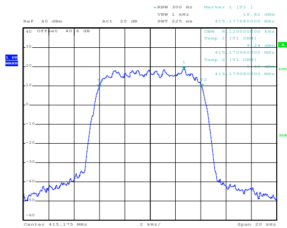
Figure 8.4-5: UL P25 input
