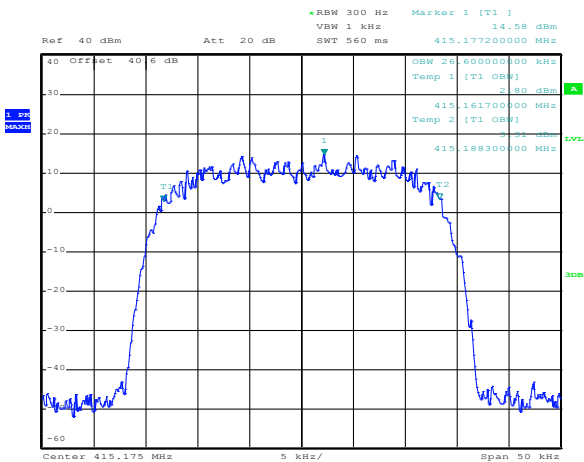
Figure 8.4-1: UL TETRA input
