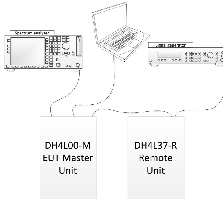
Figure 3.6-1: Setup diagram
