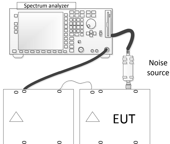
Figure 3.6-2: Noise figure setup diagram
