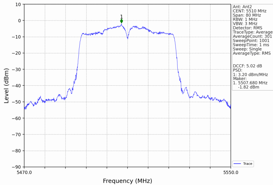
802.11n(HT40)_LCH_5510MHz_MIMO_NTNV
