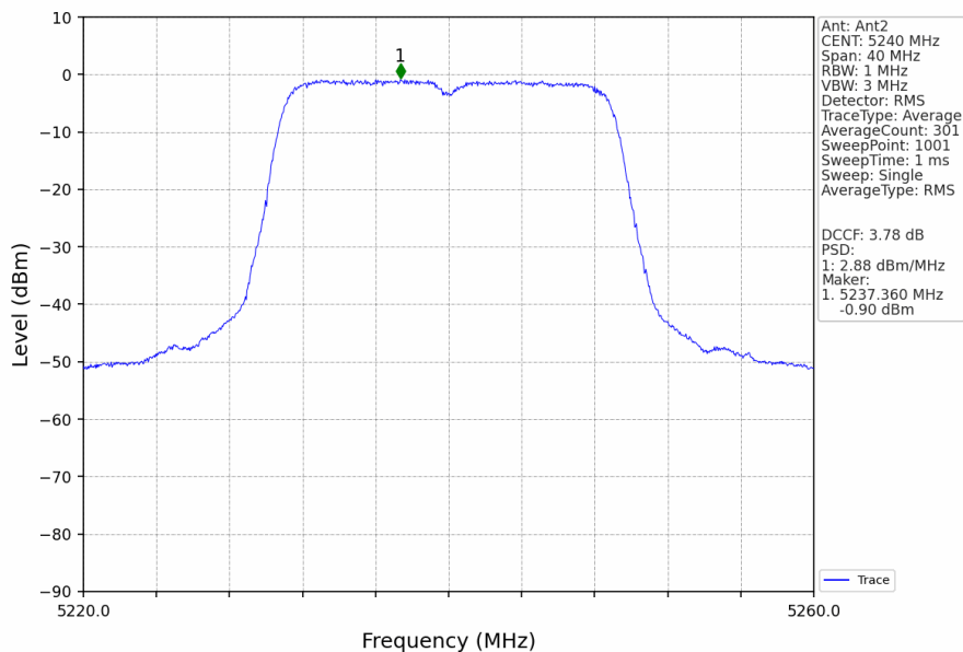
802.11ac(VHT20)_HCH_5240MHz_Ant2_NTNV
