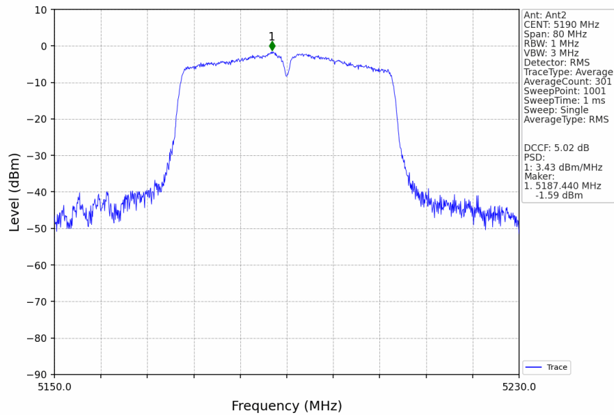
802.11n(HT40)_LCH_5190MHz_MIMO_NTNV
