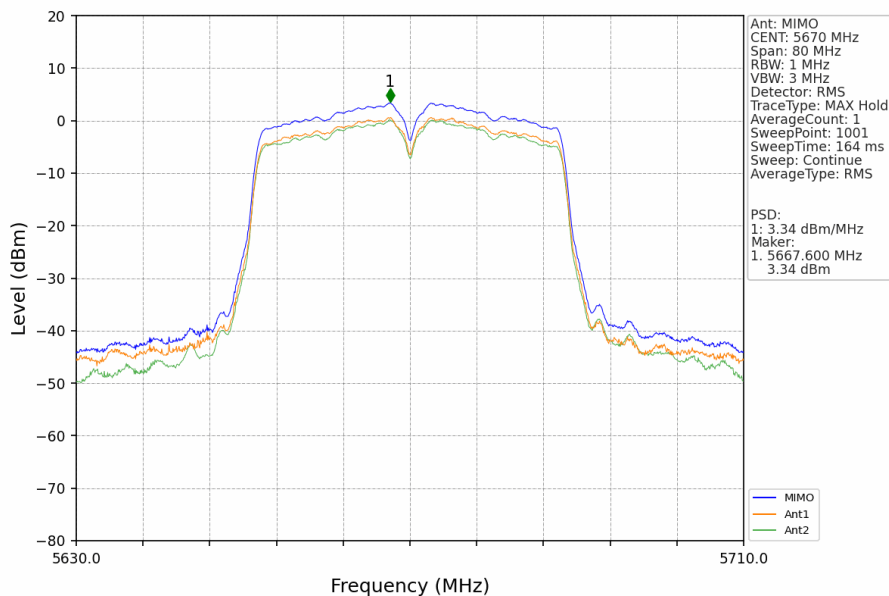
802.11n(HT40)_HCH_5670MHz_MIMO_NTNV
