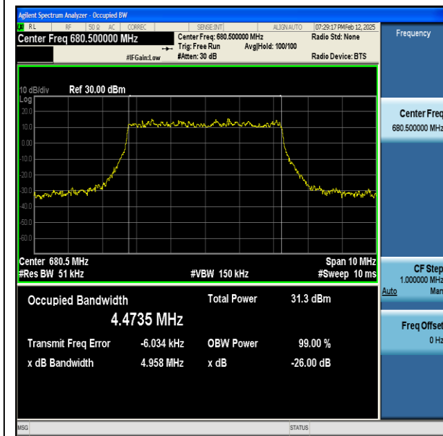
NTNV-n71-PC3-15-5-M-DFT-QPSK-Outer_Full-Ant1-PASS
