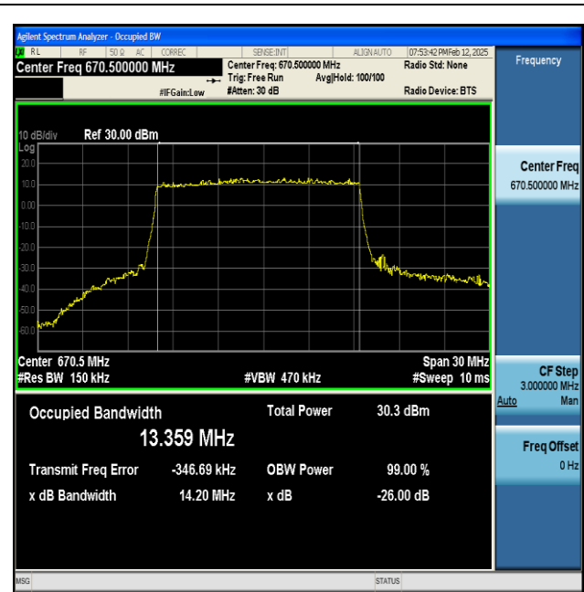
NTNV-n71-PC3-15-15-L-DFT-64QAM-Outer_Full-Ant1-PASS
