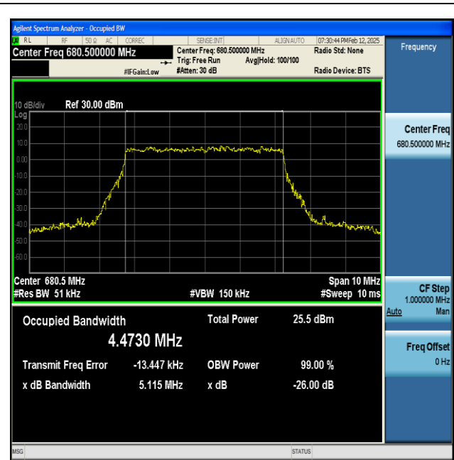
NTNV-n71-PC3-15-5-M-CP-256QAM-Outer_Full-Ant1-PASS
