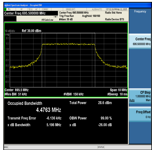
NTNV-n71-PC3-15-5-H-CP-QPSK-Outer_Full-Ant1-PASS
