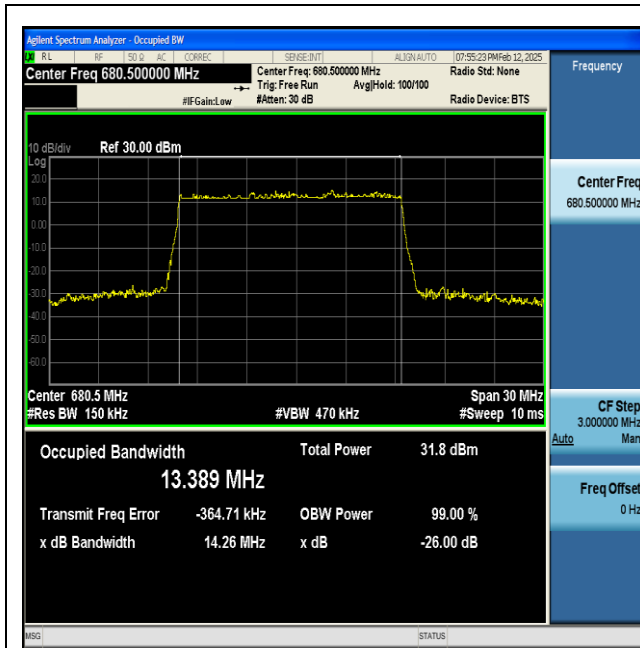
NTNV-n71-PC3-15-15-M-DFT-QPSK-Outer_Full-Ant1-PASS
