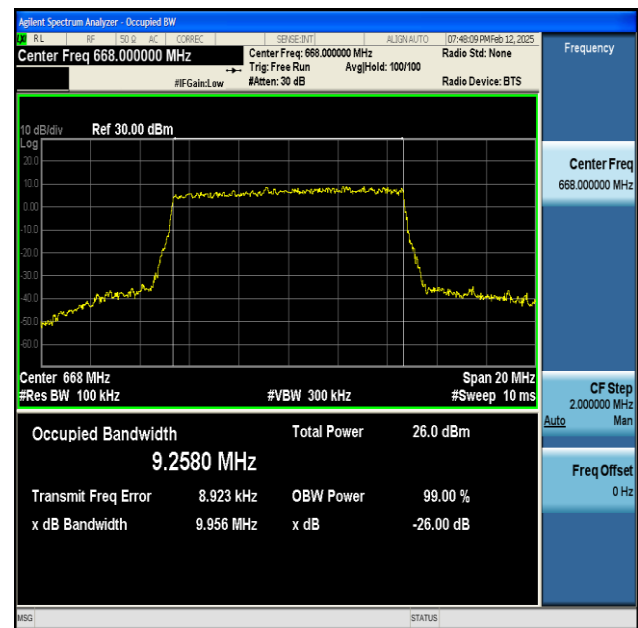
NTNV-n71-PC3-15-10-L-CP-256QAM-Outer_Full-Ant1-PASS
