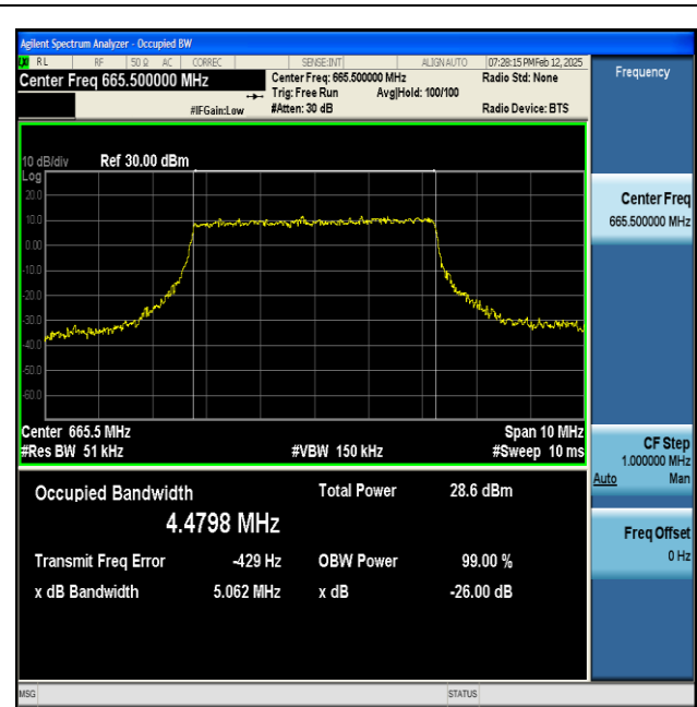
NTNV-n71-PC3-15-5-L-CP-QPSK-Outer_Full-Ant1-PASS
