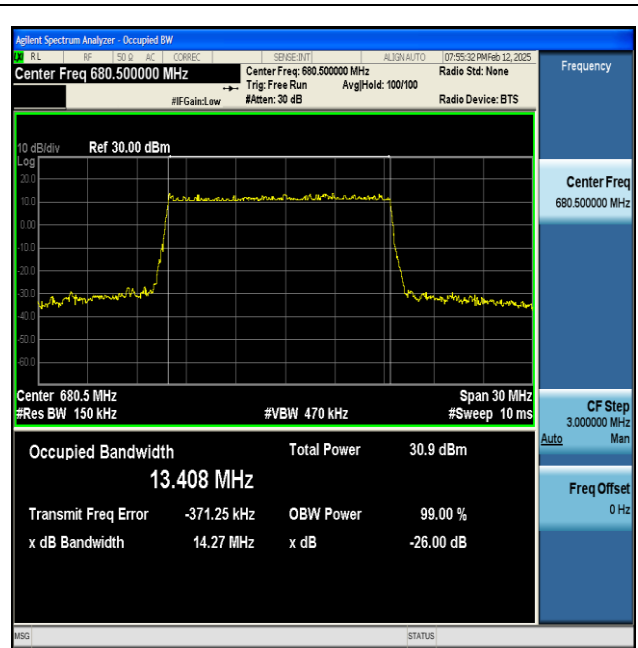
NTNV-n71-PC3-15-15-M-DFT-16QAM-Outer_Full-Ant1-PASS
