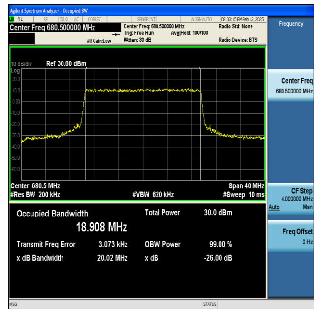
NTNV-n71-PC3-15-20-M-CP-QPSK-Outer_Full-Ant1-PASS
