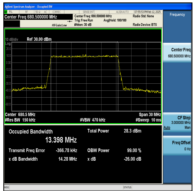
NTNV-n71-PC3-15-15-M-DFT-256QAM-Outer_Full-Ant1-PASS
