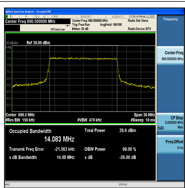
NTNV-n71-PC3-15-15-H-CP-QPSK-Outer_Full-Ant1-PASS
