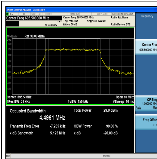
NTNV-n71-PC3-15-5-H-CP-16QAM-Outer_Full-Ant1-PASS
