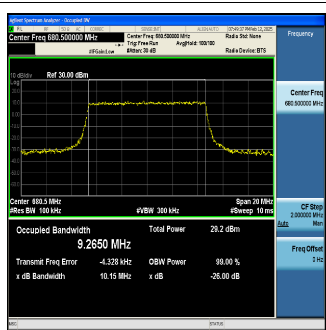
NTNV-n71-PC3-15-10-M-CP-QPSK-Outer_Full-Ant1-PASS
