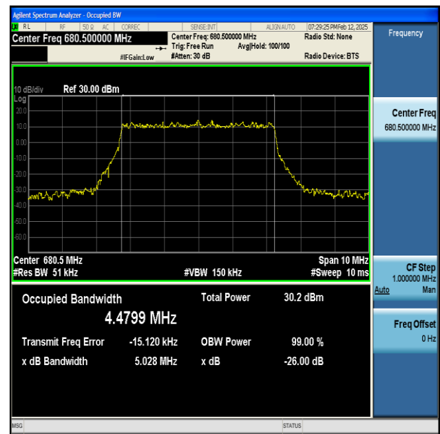
NTNV-n71-PC3-15-5-M-DFT-16QAM-Outer_Full-Ant1-PASS
