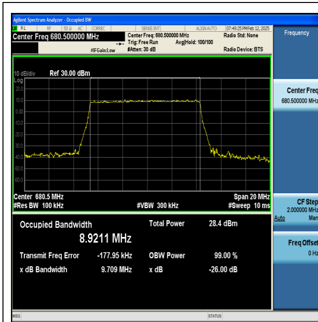
NTNV-n71-PC3-15-10-M-DFT-256QAM-Outer_Full-Ant1-PASS
