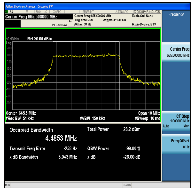
NTNV-n71-PC3-15-5-L-CP-64QAM-Outer_Full-Ant1-PASS
