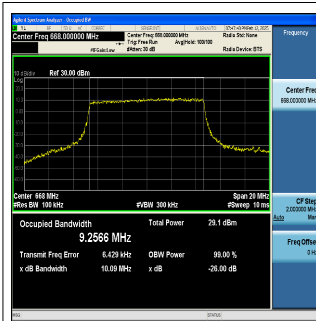
NTNV-n71-PC3-15-10-L-CP-QPSK-Outer_Full-Ant1-PASS
