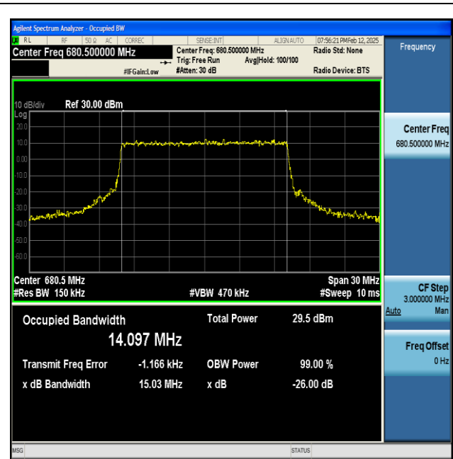
NTNV-n71-PC3-15-15-M-CP-16QAM-Outer_Full-Ant1-PASS
