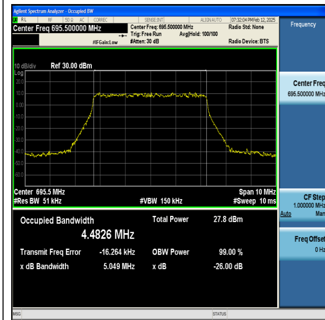
NTNV-n71-PC3-15-5-H-DFT-256QAM-Outer_Full-Ant1-PASS
