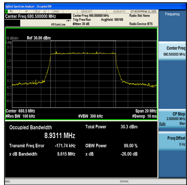
NTNV-n71-PC3-15-10-M-DFT-64QAM-Outer_Full-Ant1-PASS
