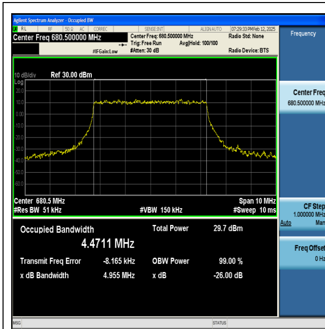
NTNV-n71-PC3-15-5-M-DFT-64QAM-Outer_Full-Ant1-PASS
