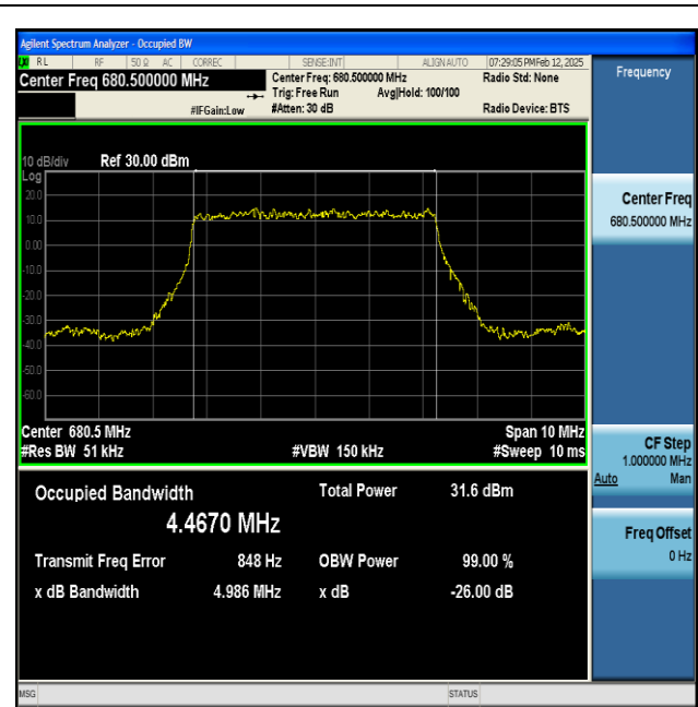
NTNV-n71-PC3-15-5-M-DFT-BPSK-Outer_Full-Ant1-PASS
