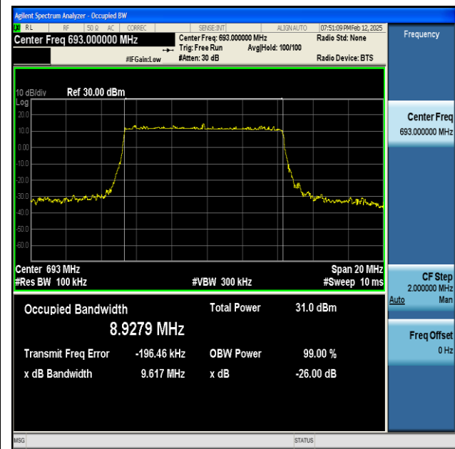
NTNV-n71-PC3-15-10-H-DFT-16QAM-Outer_Full-Ant1-PASS
