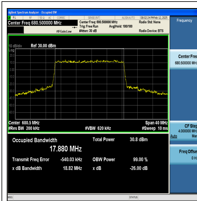
NTNV-n71-PC3-15-20-M-DFT-16QAM-Outer_Full-Ant1-PASS
