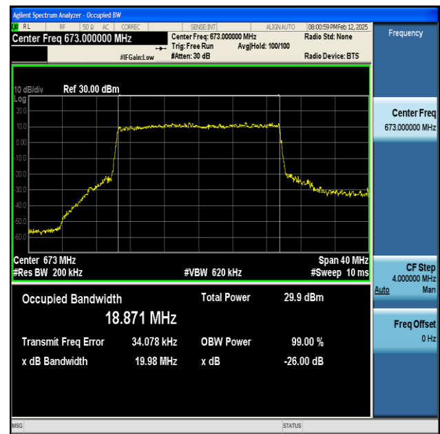
NTNV-n71-PC3-15-20-L-CP-16QAM-Outer_Full-Ant1-PASS
