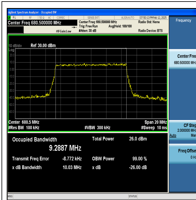
NTNV-n71-PC3-15-10-M-CP-256QAM-Outer_Full-Ant1-PASS
