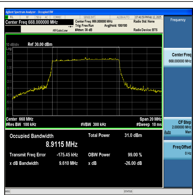
NTNV-n71-PC3-15-10-L-DFT-16QAM-Outer_Full-Ant1-PASS
