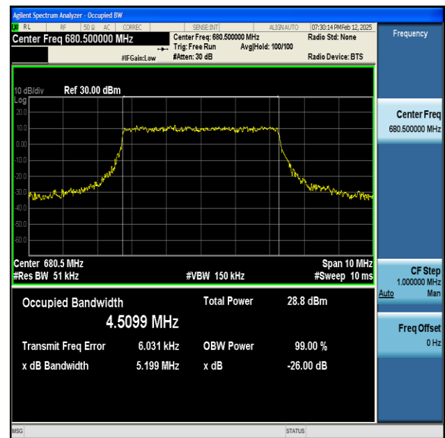
NTNV-n71-PC3-15-5-M-CP-16QAM-Outer_Full-Ant1-PASS
