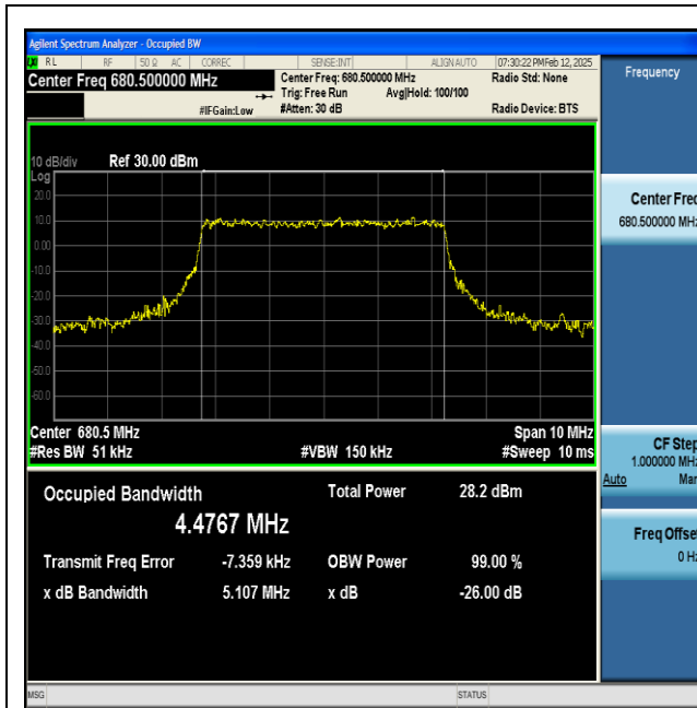
NTNV-n71-PC3-15-5-M-CP-64QAM-Outer_Full-Ant1-PASS
