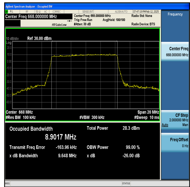
NTNV-n71-PC3-15-10-L-DFT-256QAM-Outer_Full-Ant1-PASS
