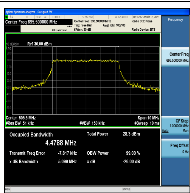
NTNV-n71-PC3-15-5-H-CP-64QAM-Outer_Full-Ant1-PASS
