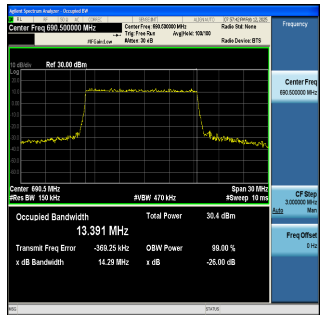
NTNV-n71-PC3-15-15-H-DFT-64QAM-Outter_Full-Ant1-PASS
