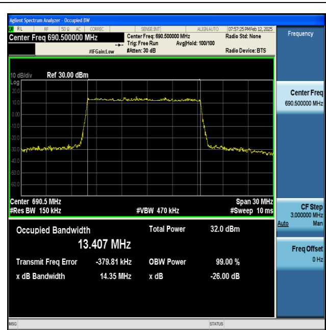
NTNV-n71-PC3-15-15-H-DFT-QPSK-Outter_Full-Ant1-PASS
