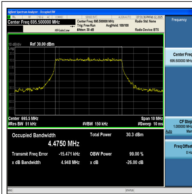
NTNV-n71-PC3-15-5-H-DFT-16QAM-Outer_Full-Ant1-PASS
