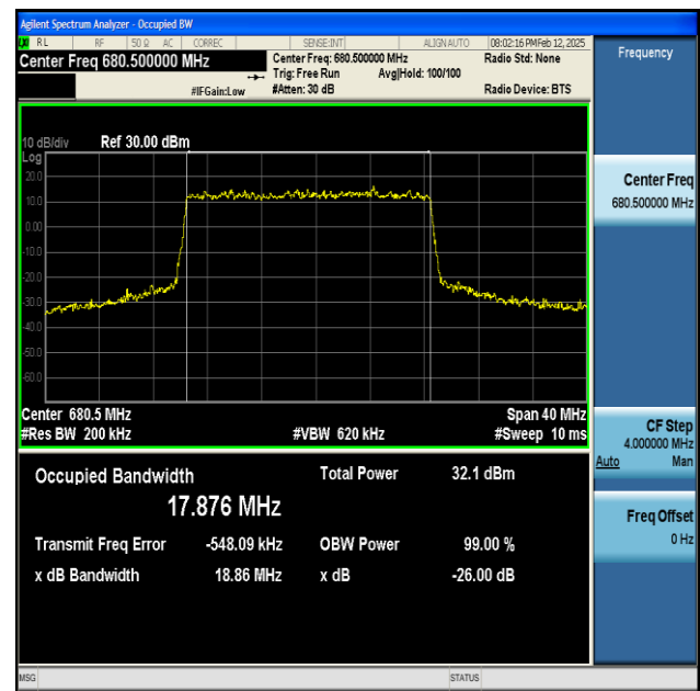
NTNV-n71-PC3-15-20-M-DFT-QPSK-Outer_Full-Ant1-PASS
