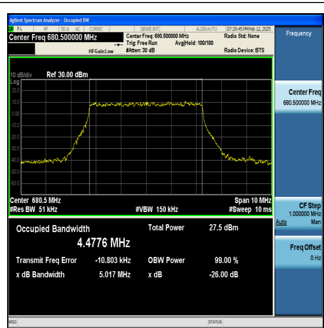
NTNV-n71-PC3-15-5-M-DFT-256QAM-Outer_Full-Ant1-PASS
