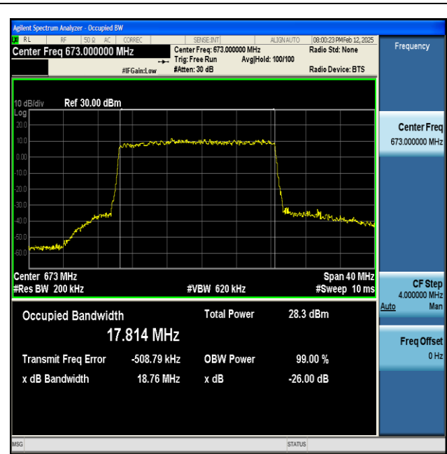
NTNV-n71-PC3-15-20-L-DFT-256QAM-Outer_Full-Ant1-PASS
