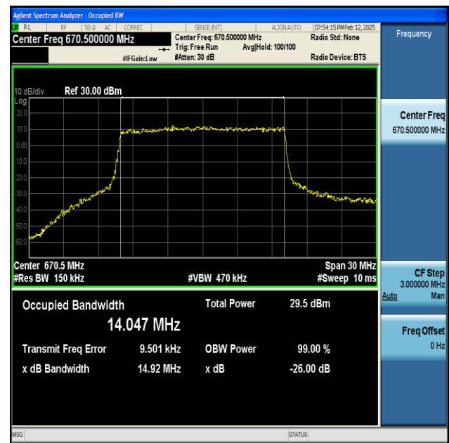
NTNV-n71-PC3-15-15-L-CP-QPSK-Outer_Full-Ant1-PASS
