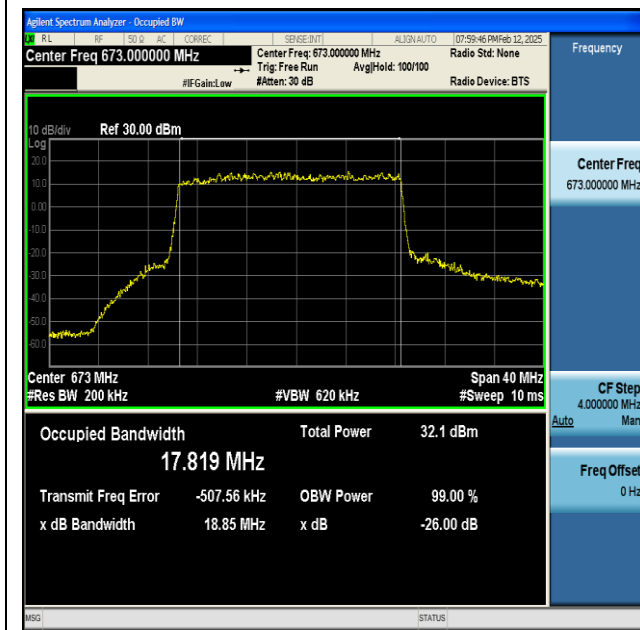
NTNV-n71-PC3-15-20-L-DFT-QPSK-Outer_Full-Ant1-PASS
