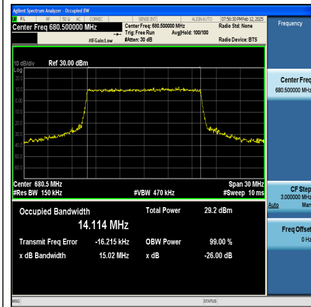
NTNV-n71-PC3-15-15-M-CP-64QAM-Outer_Full-Ant1-PASS
