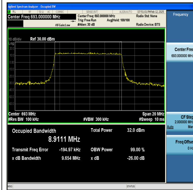
NTNV-n71-PC3-15-10-H-DFT-QPSK-Outer_Full-Ant1-PASS
