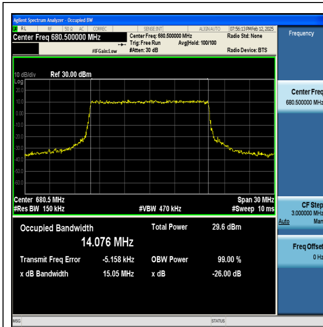
NTNV-n71-PC3-15-15-M-CP-QPSK-Outer_Full-Ant1-PASS
