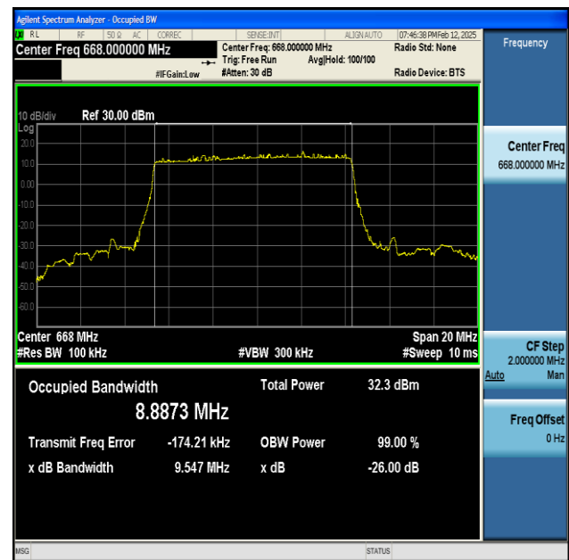
NTNV-n71-PC3-15-10-L-DFT-BPSK-Outer_Full-Ant1-PASS
