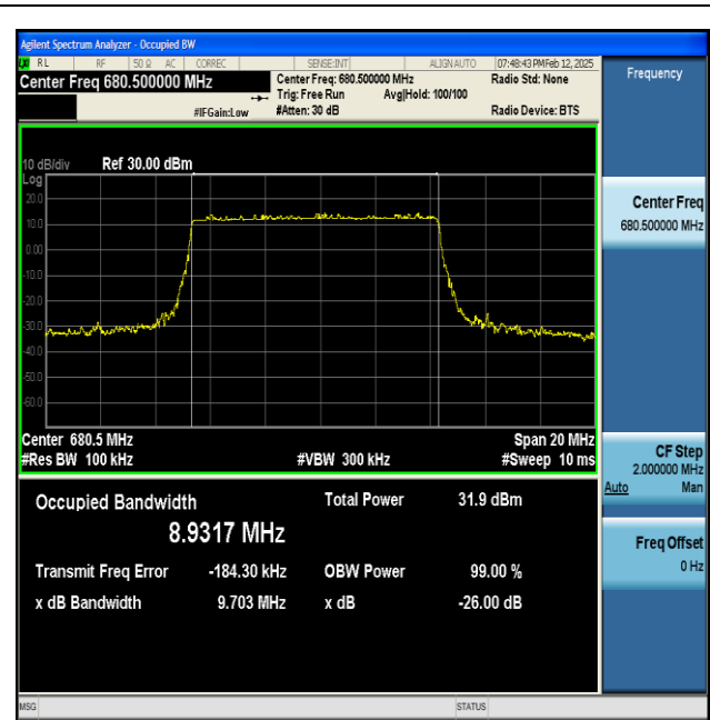
NTNV-n71-PC3-15-10-M-DFT-QPSK-Outer_Full-Ant1-PASS
