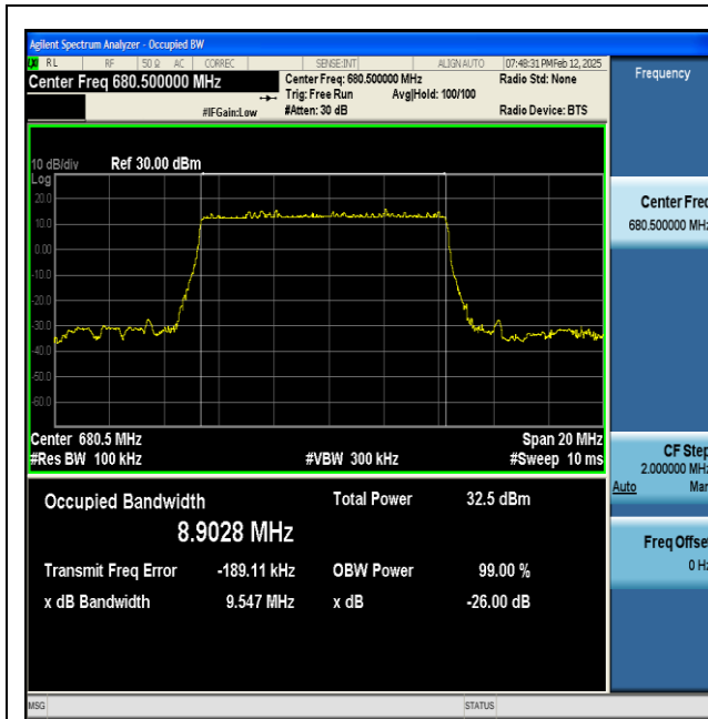
NTNV-n71-PC3-15-10-M-DFT-BPSK-Outer_Full-Ant1-PASS
