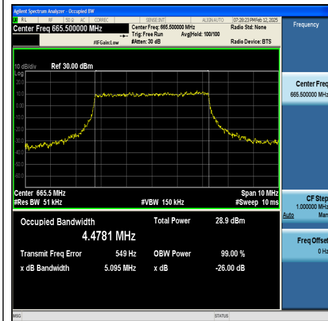
TNV-n71-PC3-15-5-L-CP-16QAM-Outer_Full-Ant1-PASS
