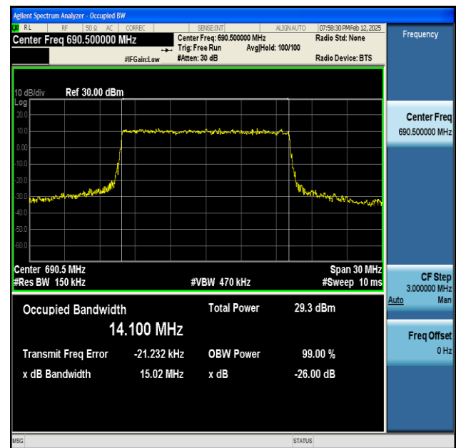
NTNV-n71-PC3-15-15-H-CP-64QAM-Outer_Full-Ant1-PASS
