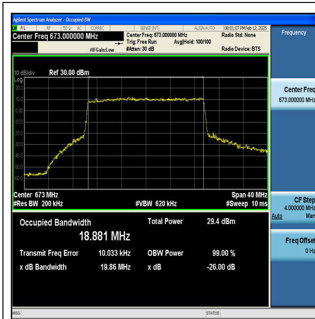
NTNV-n71-PC3-15-20-L-CP-64QAM-Outer_Full-Ant1-PASS
