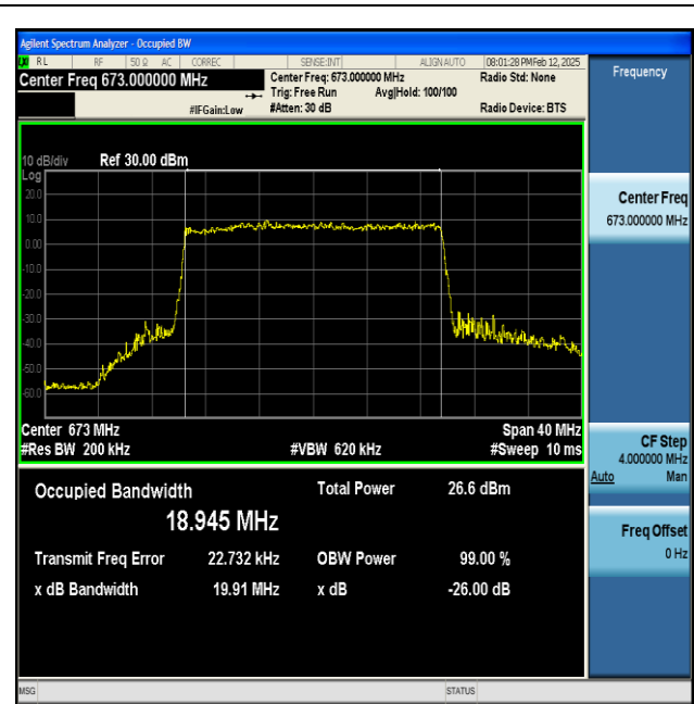
NTNV-n71-PC3-15-20-L-CP-256QAM-Outer_Full-Ant1-PASS
