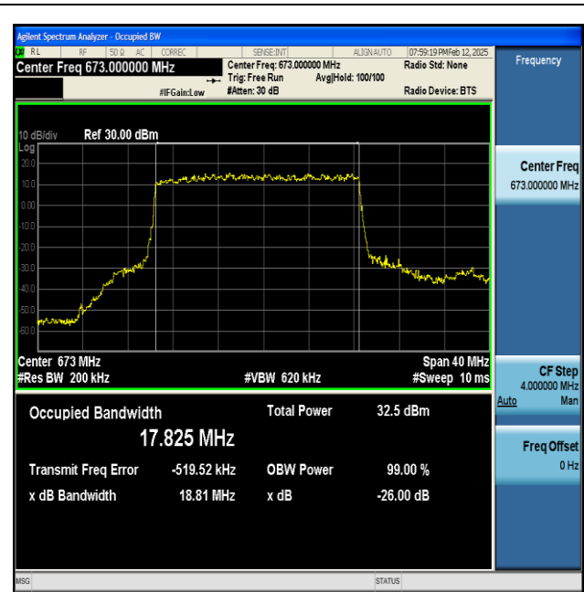
NTNV-n71-PC3-15-20-L-DFT-BPSK-Outer_Full-Ant1-PASS
