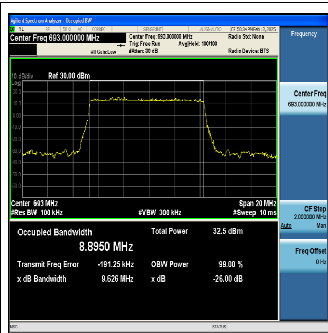
NTNV-n71-PC3-15-10-H-DFT-BPSK-Outer_Full-Ant1-PASS
