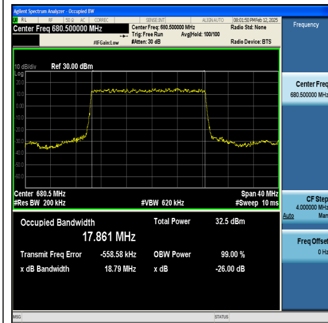
NTNV-n71-PC3-15-20-M-DFT-BPSK-Outer_Full-Ant1-PASS
