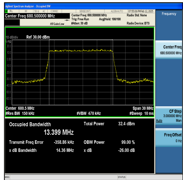
NTNV-n71-PC3-15-15-M-DFT-BPSK-Outer_Full-Ant1-PASS
