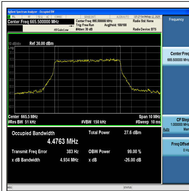
NTNV-n71-PC3-15-5-L-DFT-256QAM-Outer_Full-Ant1-PASS
