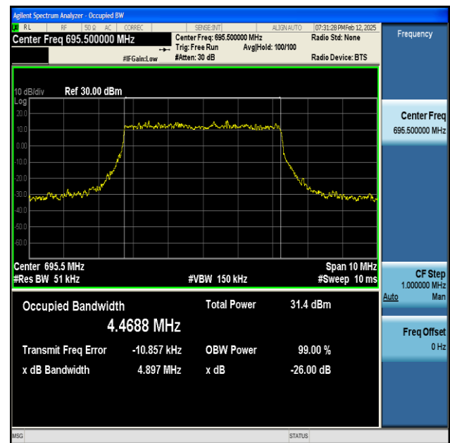
NTNV-n71-PC3-15-5-H-DFT-QPSK-Outer_Full-Ant1-PASS
