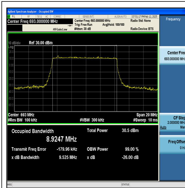
NTNV-n71-PC3-15-10-H-DFT-64QAM-Outer_Full-Ant1-PASS
