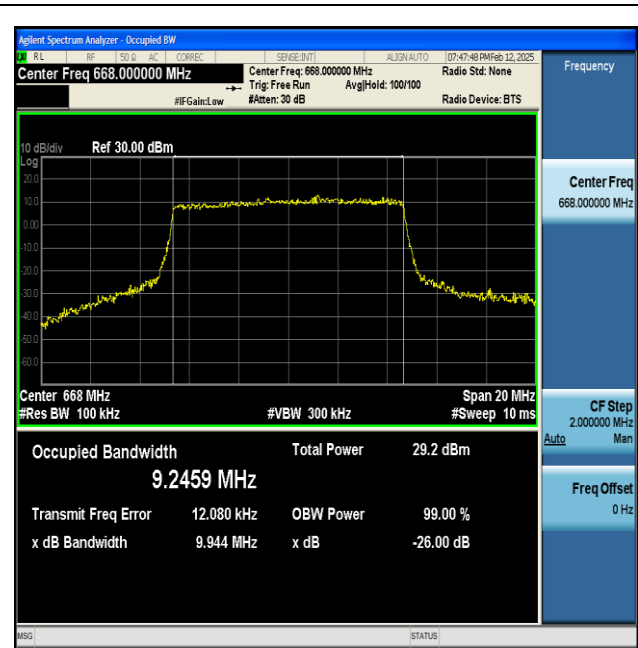
NTNV-n71-PC3-15-10-L-CP-16QAM-Outer_Full-Ant1-PASS
