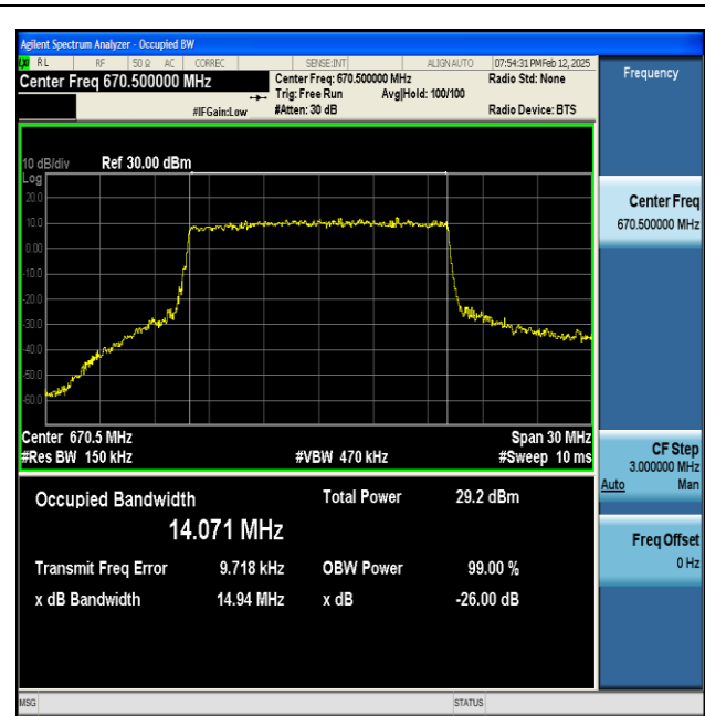
NTNV-n71-PC3-15-15-L-CP-64QAM-Outer_Full-Ant1-PASS
