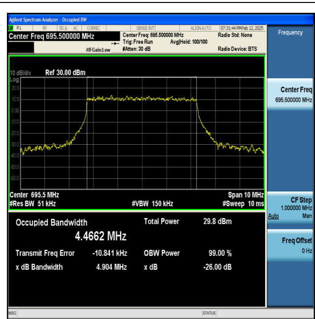
NTNV-n71-PC3-15-5-H-DFT-64QAM-Outer_Full-Ant1-PASS
