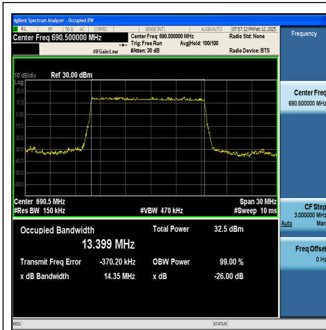
NTNV-n71-PC3-15-15-H-DFT-BPSK-Outter_Full-Ant1-PASS
