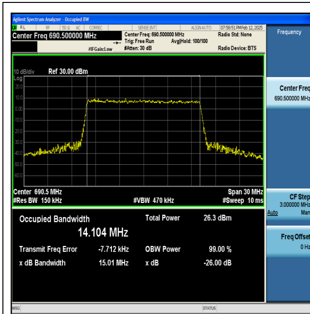
NTNV-n71-PC3-15-15-H-CP-256QAM-Outer_Full-Ant1-PASS
