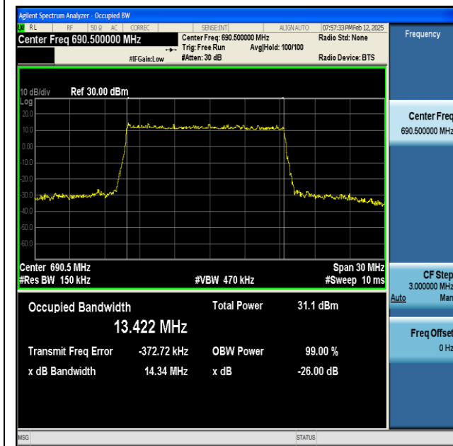
NTNV-n71-PC3-15-15-H-DFT-16QAM-Outter_Full-Ant1-PASS
