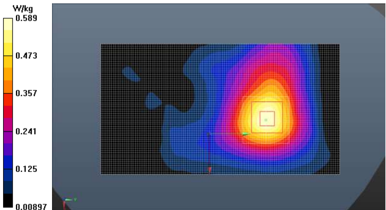
Fig.32 LTE Band 41
