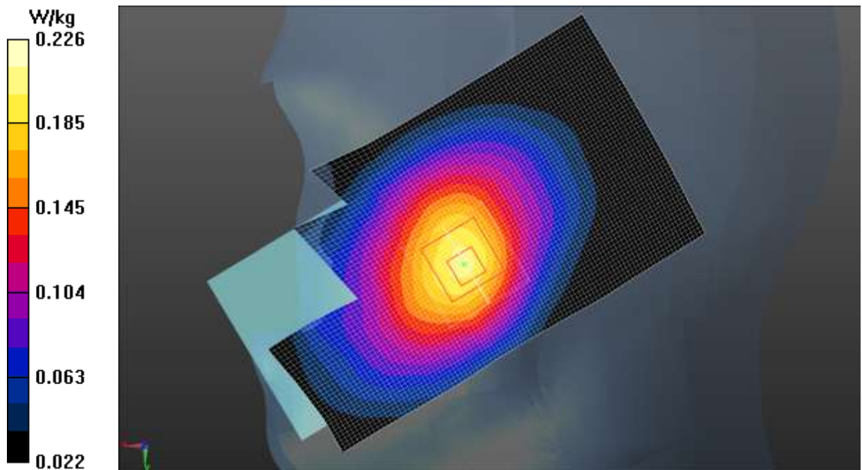
Fig.25 LTE Band 13
