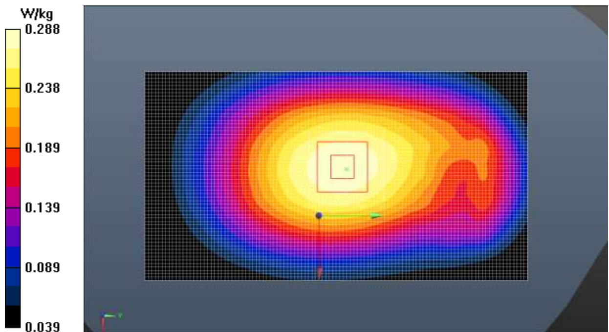
Fig.24 LTE Band 12
