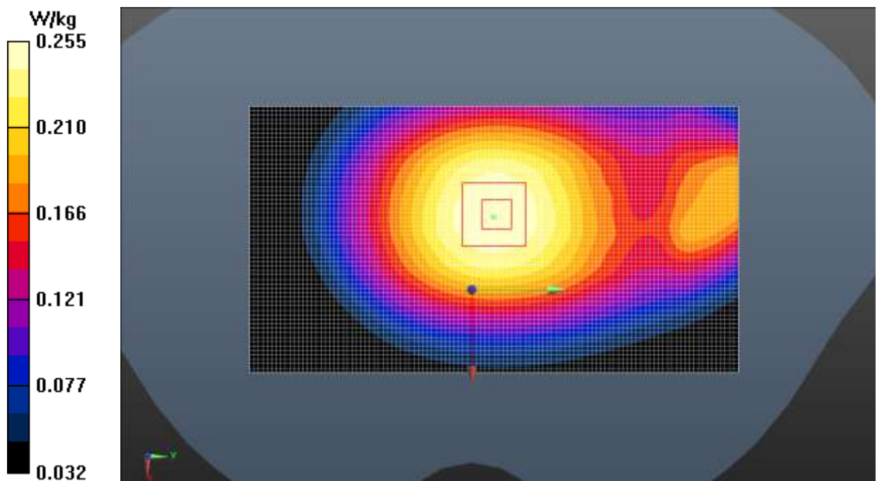
Fig.10 CDMA BC10
