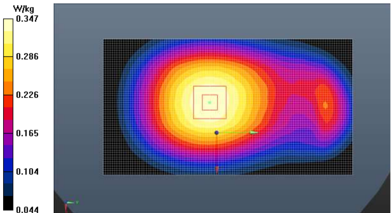
Fig.30 LTE Band 26
