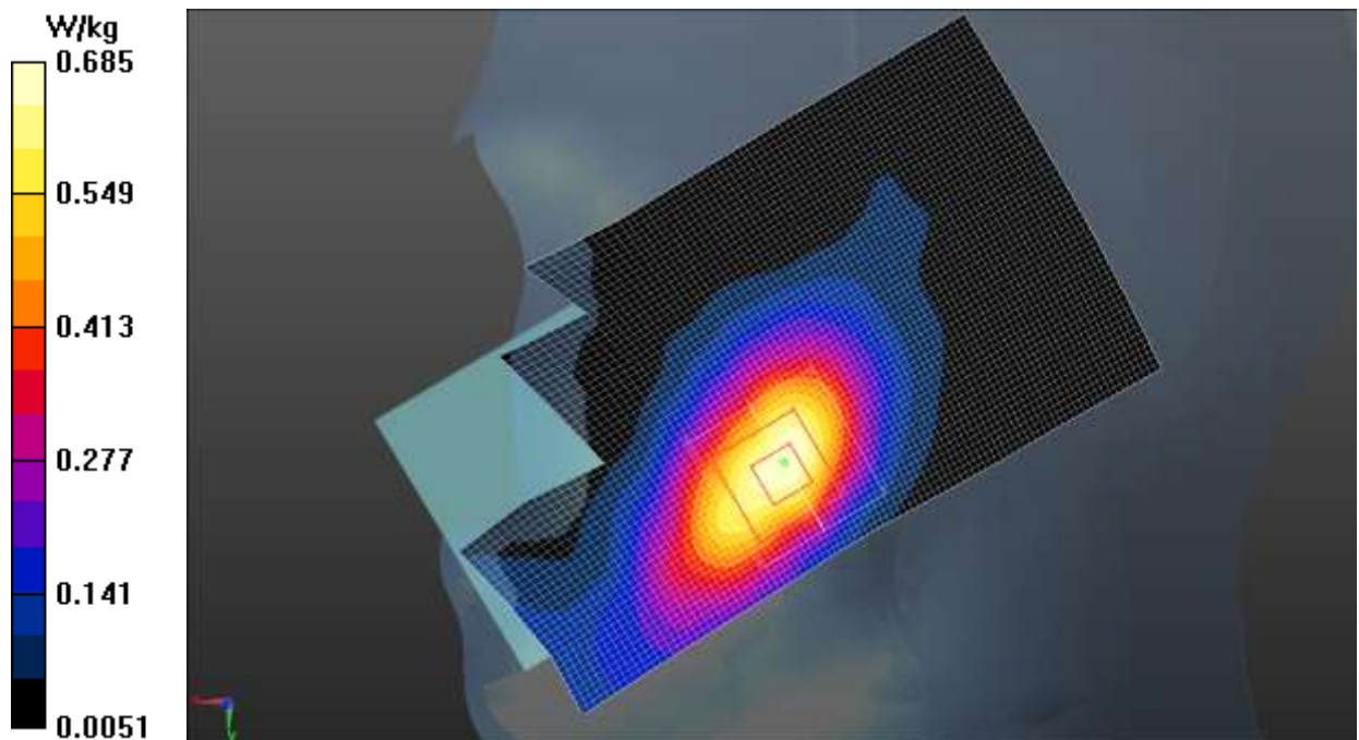
Fig.17 LTE Band 2
