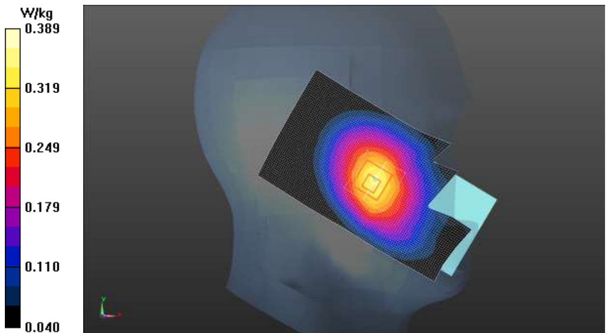
Fig.11 WCDMA 850
