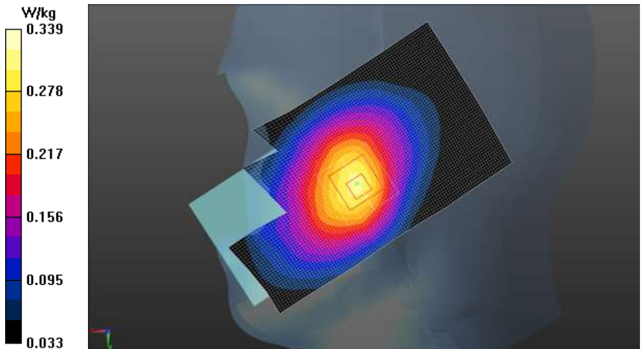
Fig.29 LTE Band 26
