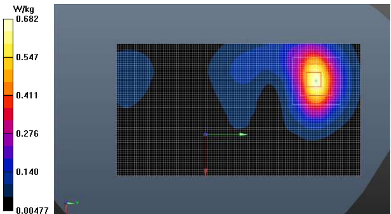
Fig.16 WCDMA 1700
