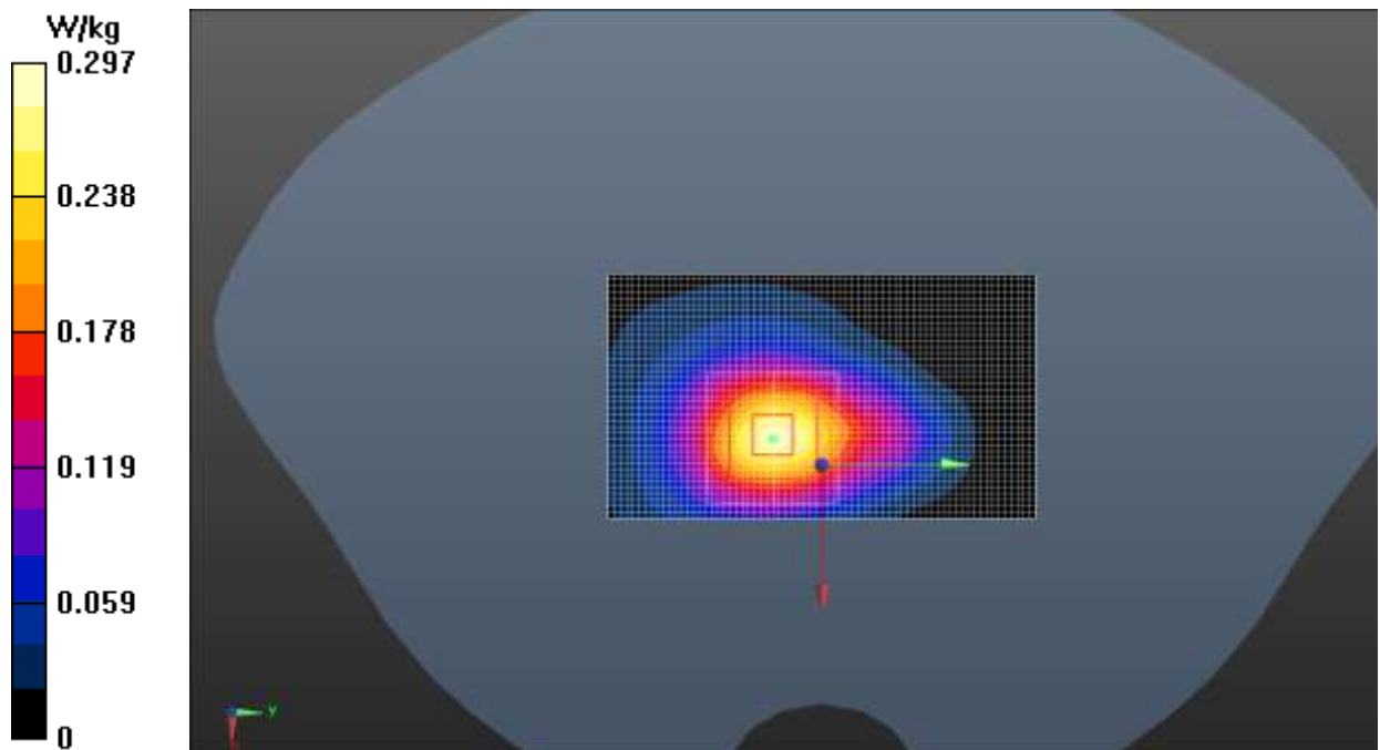
Fig.38 Wi-Fi 2.4G
