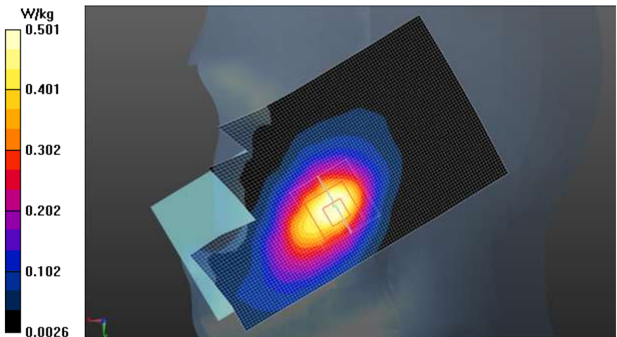
Fig.3 GSM 1900
