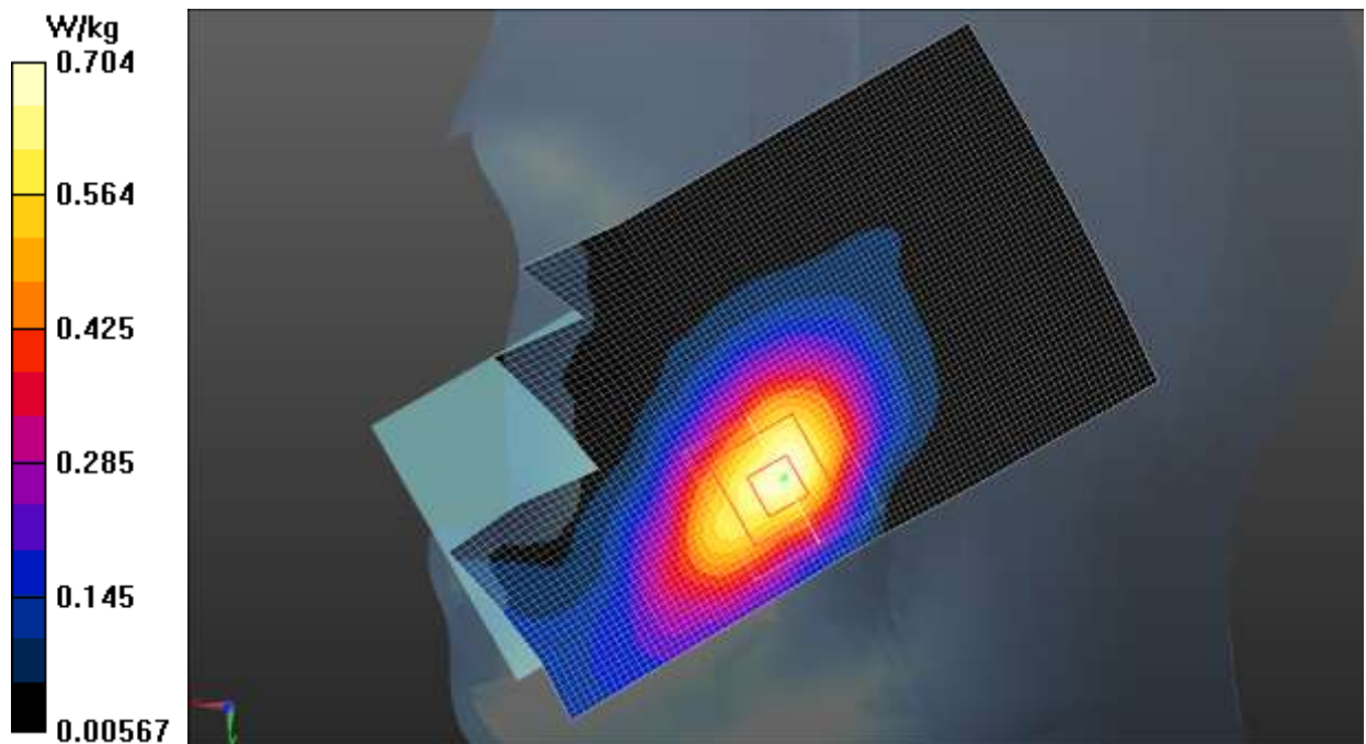
Fig.27 LTE Band 25
