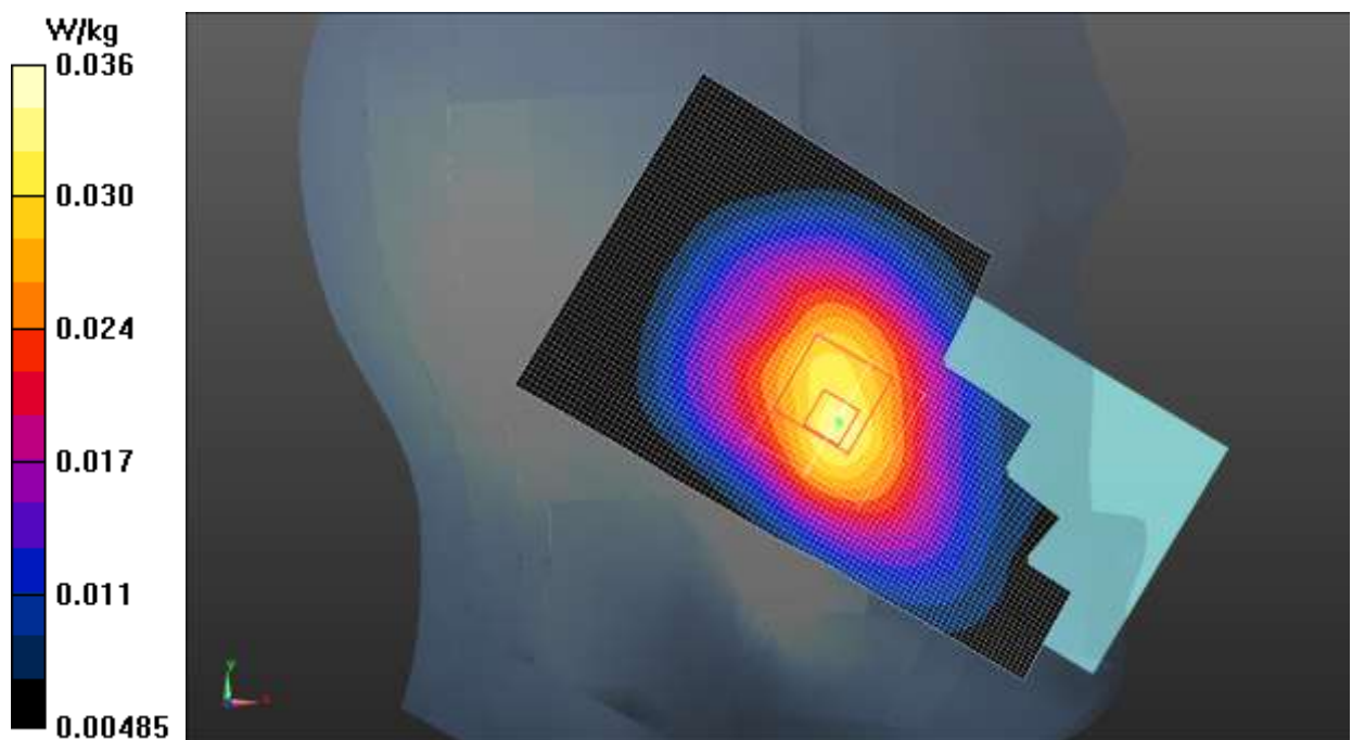
Fig.35 LTE Band 71
