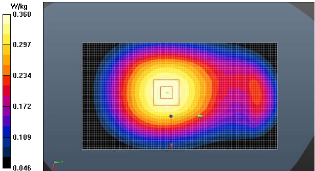
Fig.22 LTE Band 5
