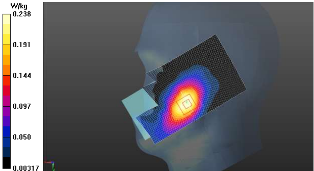
Fig.15 WCDMA 1700
