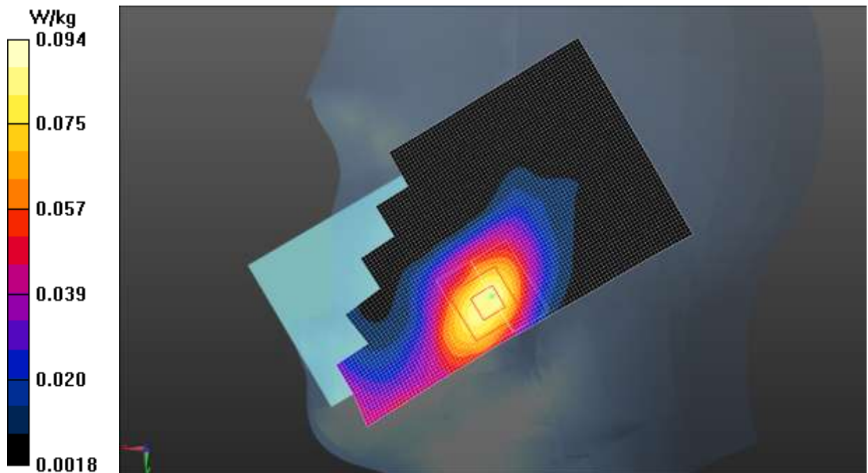
Fig.33 LTE Band 66
