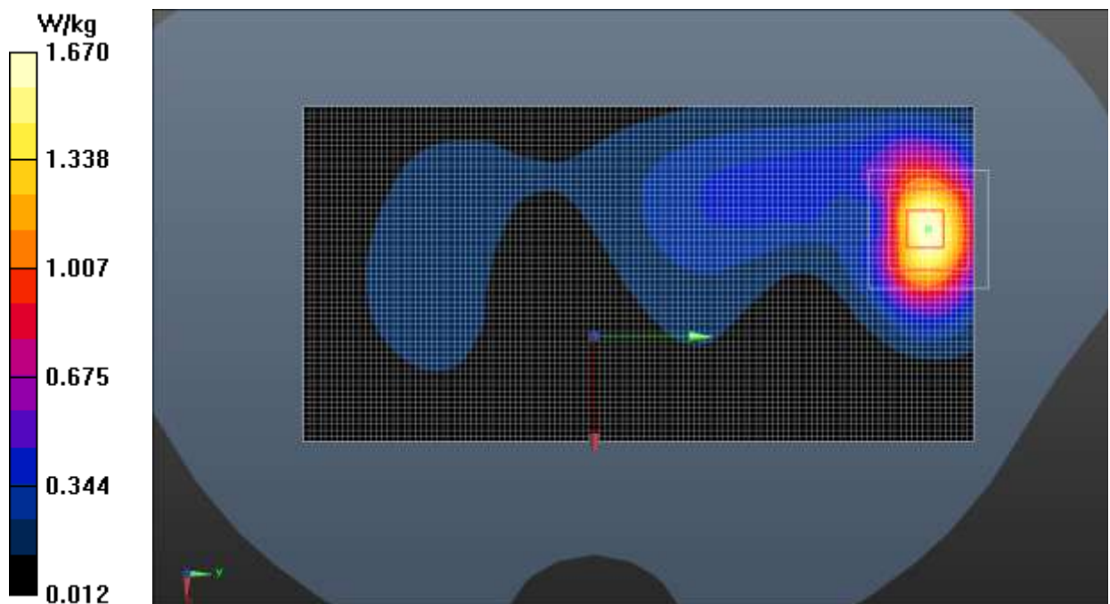
Fig.4 GSM 1900
