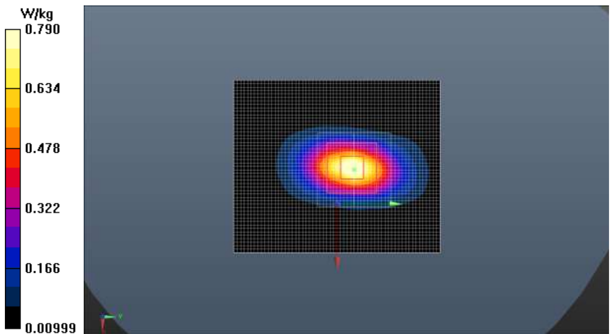
Fig.34 LTE Band 66
