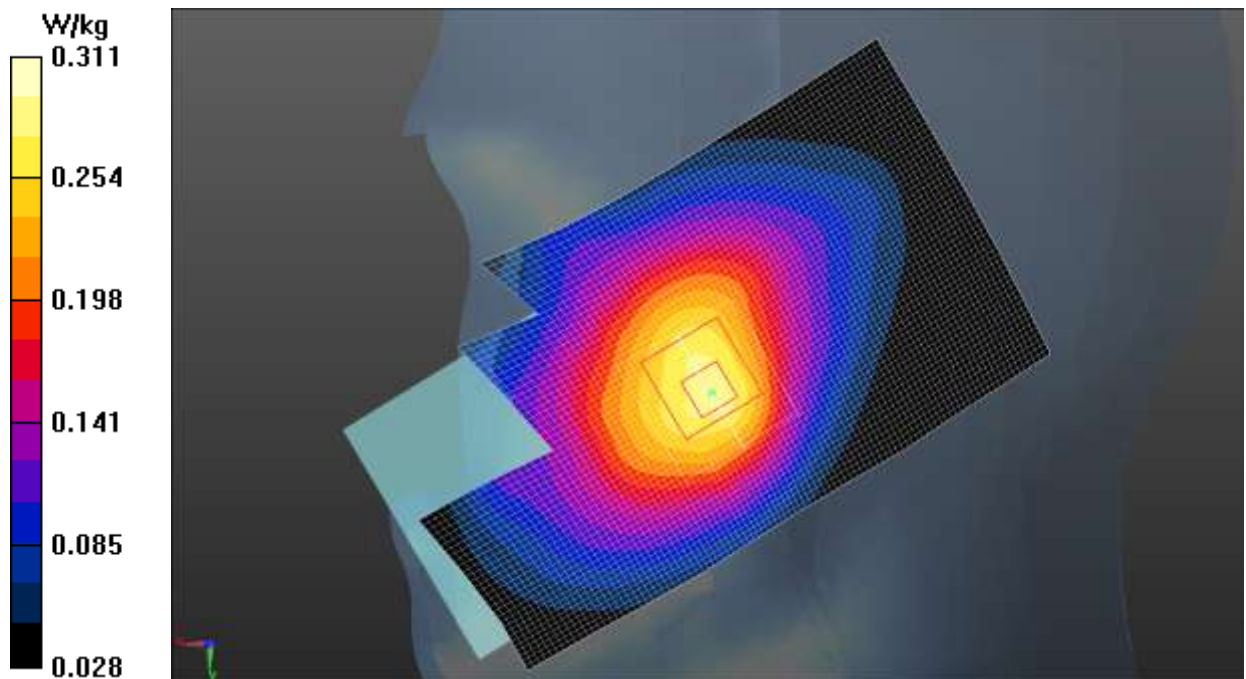
Fig.21 LTE Band 5
