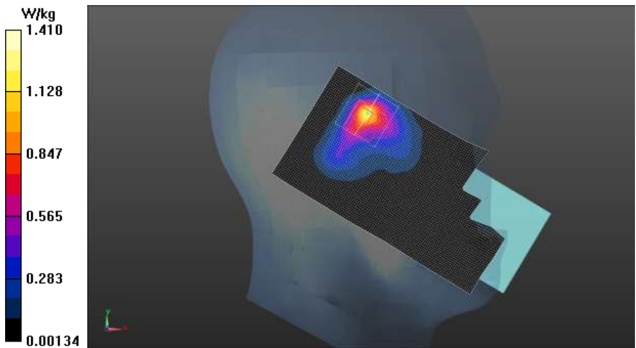
Fig.37 Wi-Fi 2.4G
