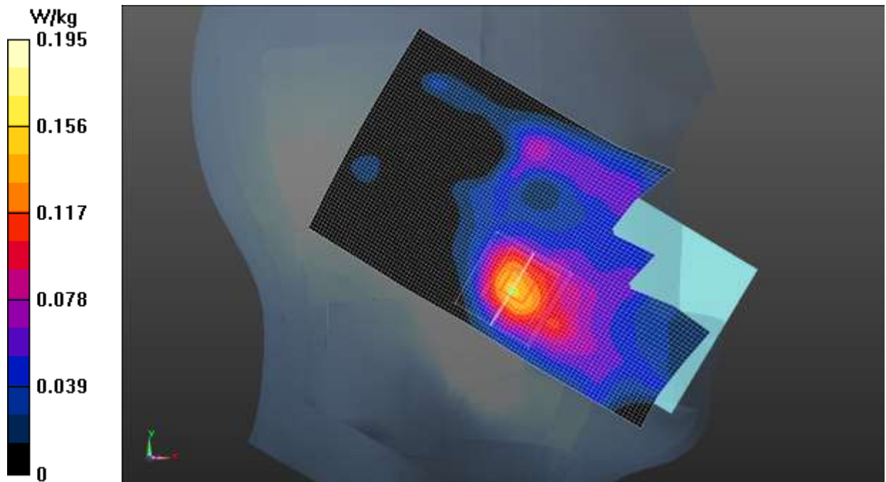
Fig.31 LTE Band 41
