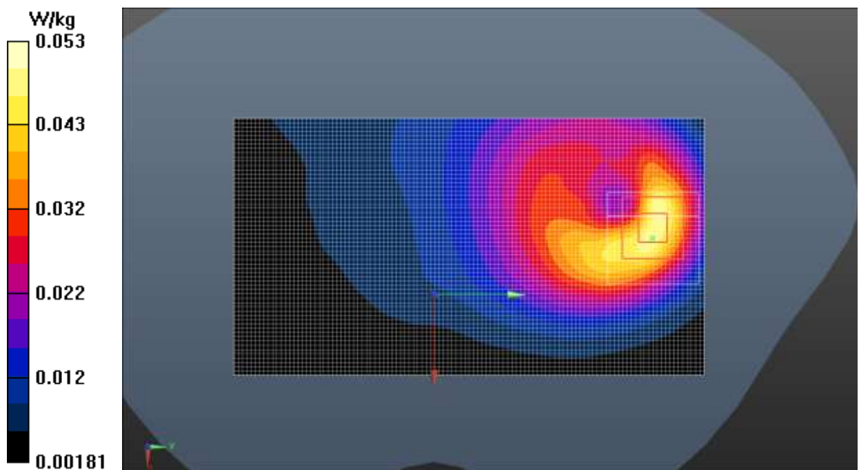
Fig.36 LTE Band 71
