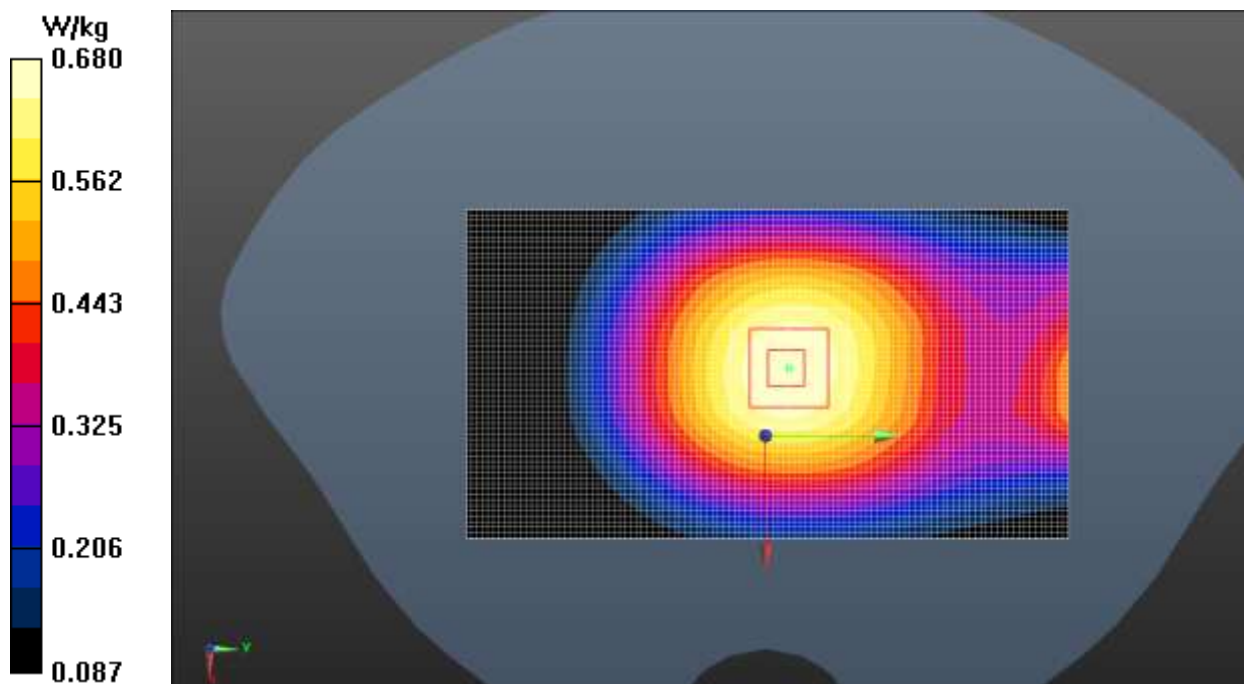
Fig.2 GSM 850
