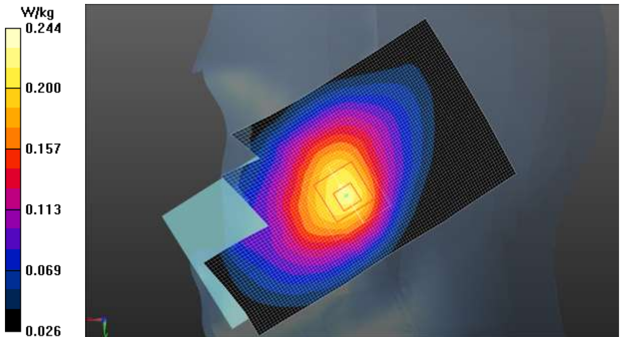
Fig.23 LTE Band 12
