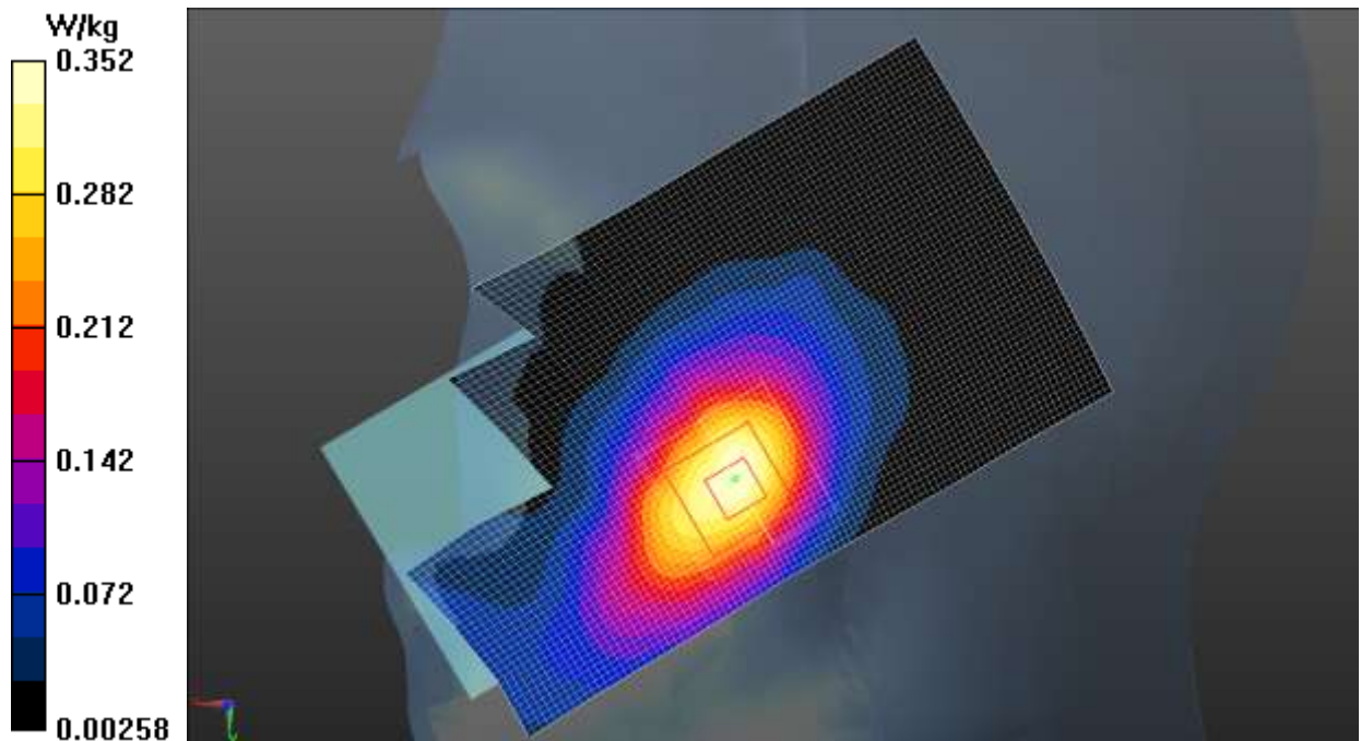
Fig.19 LTE Band 4
