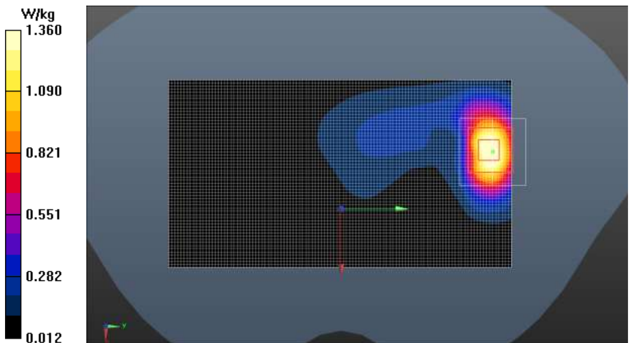
Fig.28 LTE Band 25
