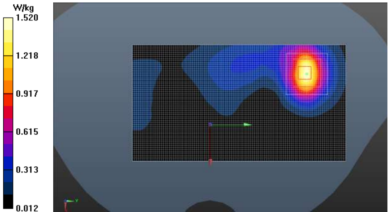
Fig.14 WCDMA 1900
