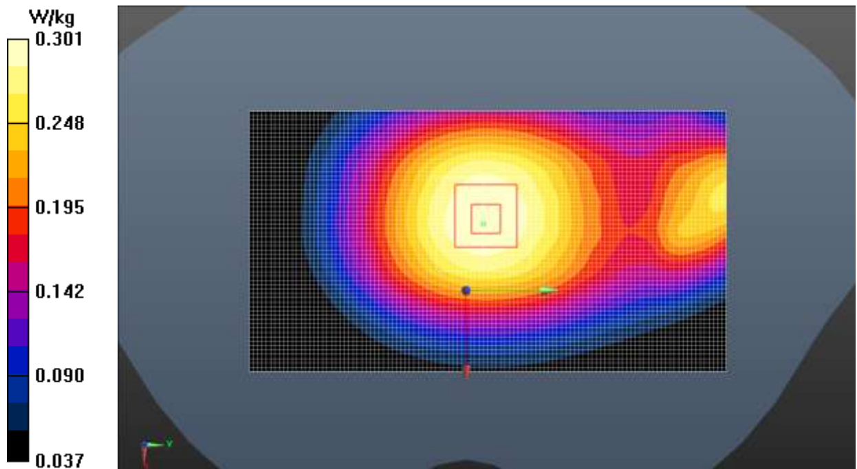
Fig.6 CDMA BC0
