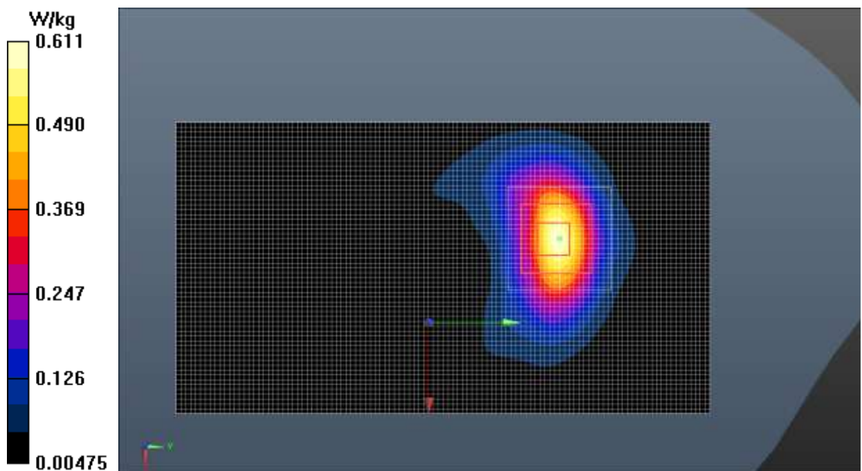
Fig.20 LTE Band 4
