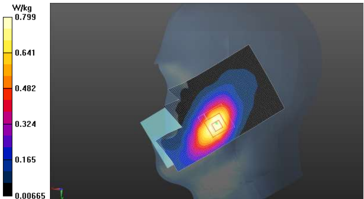
Fig.13 WCDMA 1900
