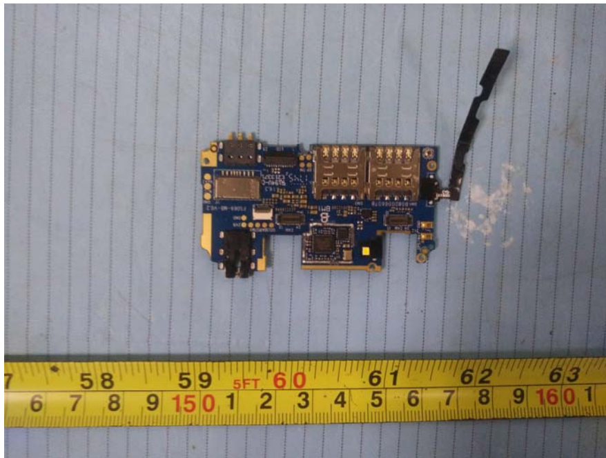
EUT – Mainboard Top Shielding off View 3
