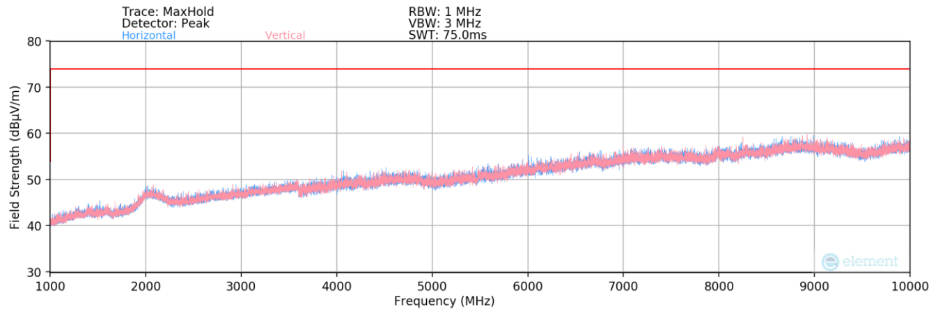
Plot 7-4. Radiated Spurious Plot above 1GHz – Half-Open
