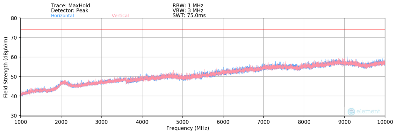
Plot 7-3. Radiated Spurious Plot above 1GHz – Closed
