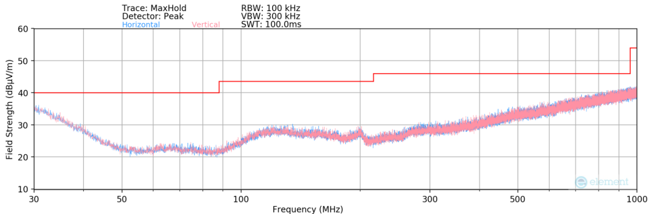
Plot 7-1. Radiated Spurious Plot below 1GHz – Closed
