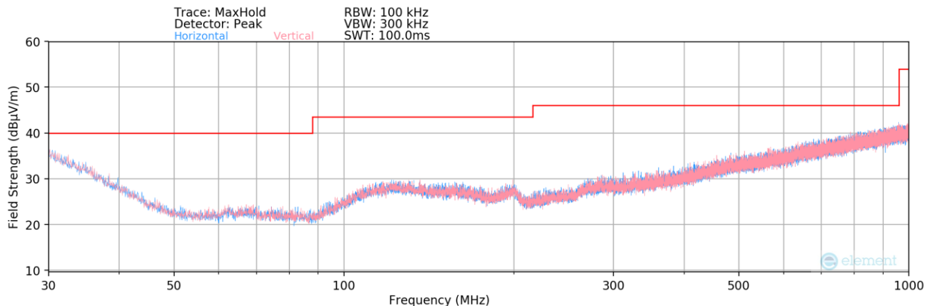
Plot 7-2. Radiated Spurious Plot below 1GHz – Half-Open
