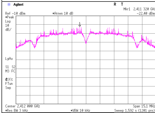
11b Antenna 1
