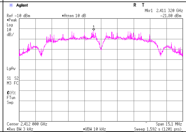
11b Antenna 2
