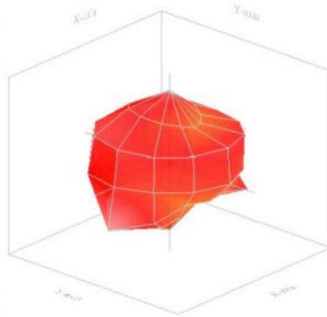
Radiation pattern
