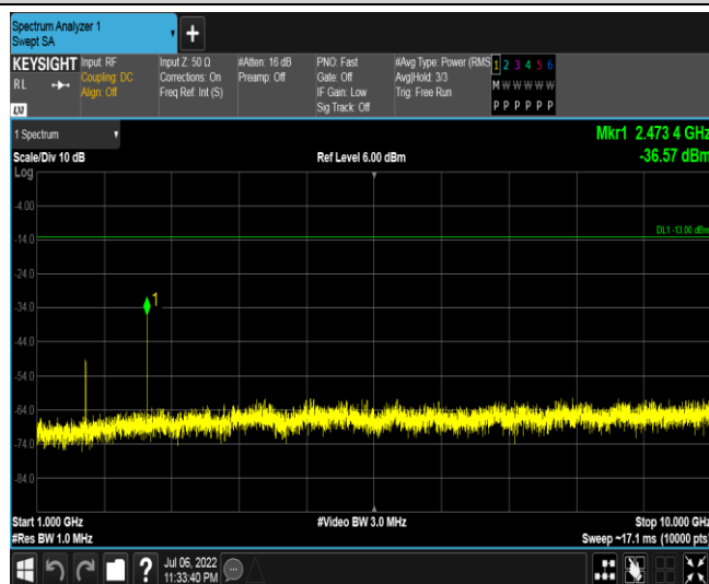
Band5-3MHz-16QAM-20415-1RB#0-Range3:1000~10000MHz
