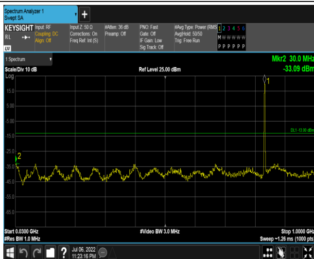
Band5-1.4MHz-16QAM-20525-1RB#0-Range2:30~1000MHz
