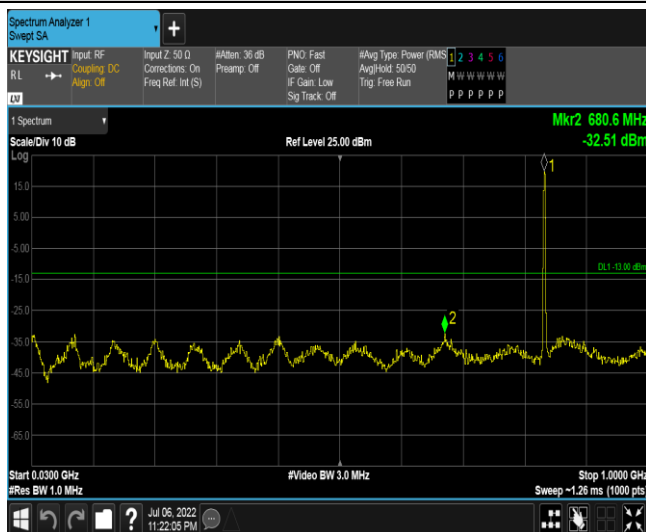
Band5-1.4MHz-QPSK-20525-1RB#0-Range2:30~1000MHz
