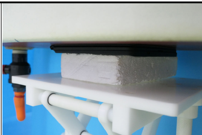
Rear Face of EUT with Holster Tested at 0 mm
