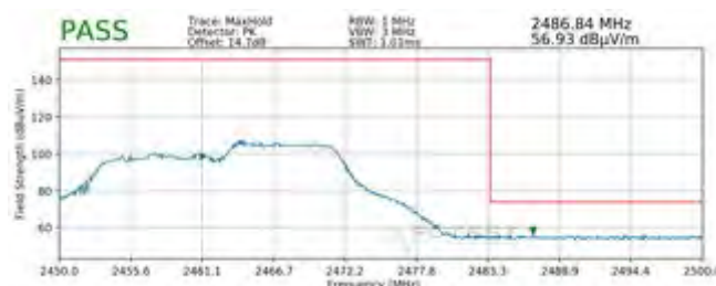
Plot 7-92. Radiated Restricted Upper Band Edge Measurement SISO ANT2 (Peak – 106 Tones)
