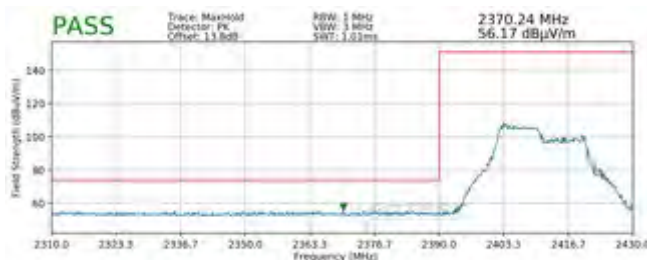
Plot 7-90. Radiated Restricted Lower Band Edge Measurement SISO ANT2 (Peak – 106 Tones)
