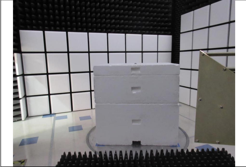
RF Radiated #3
