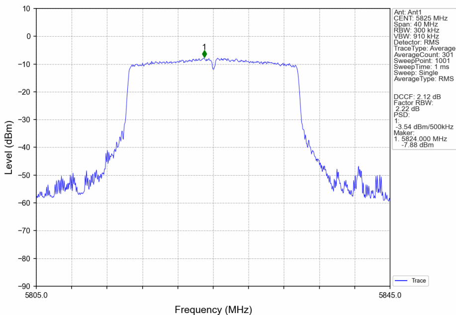
802.11ax(HEW20)_HCH_5825MHz_SU_/_Ant1_NTNV
