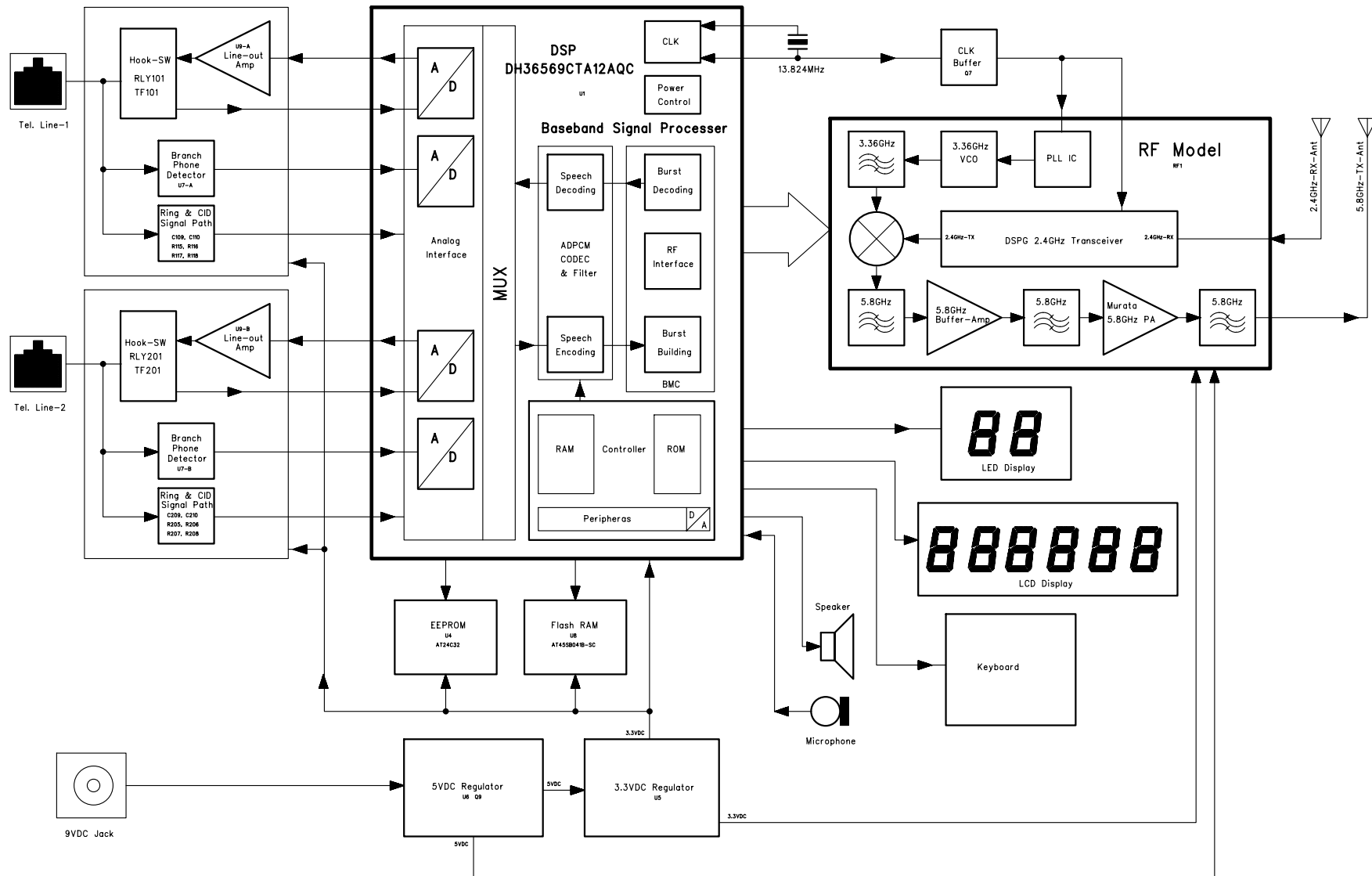
NWB35828 Base Unit Block Diagram
