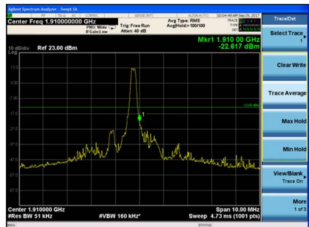
LTE Band 2 1.4MHz QPSK 1RB CH-High
