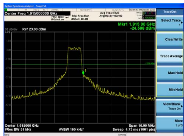
LTE Band 25 3MHz 16QAM 1RB CH-High
