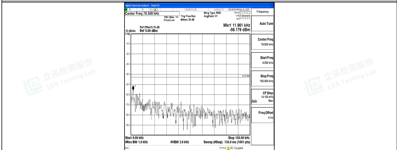
Band4_5MHz_16QAM_20175_1RB#0_0.009~0.15_0.009~0.15
