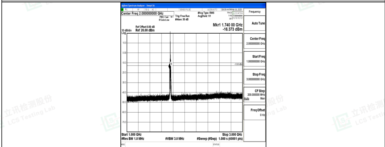
Band4_5MHz_QPSK_20375_1RB#0_1000~3000_1000~3000
