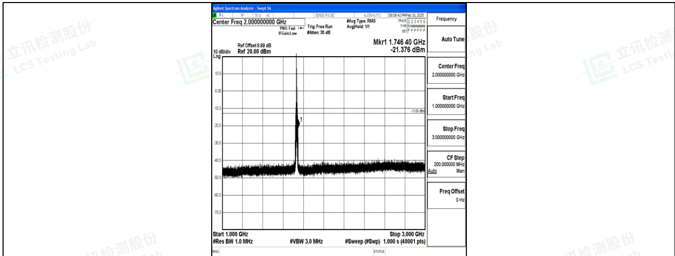
Band4_5MHz_QPSK_20175_1RB#0_1000~3000_1000~3000
