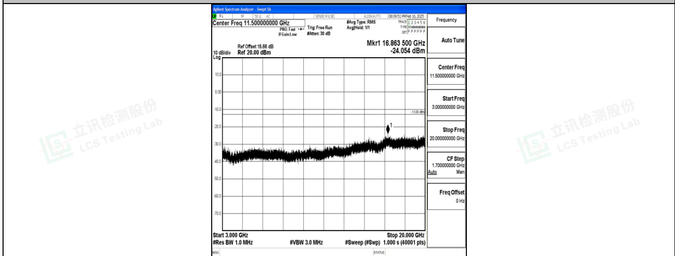
Band4_5MHz_QPSK_20375_1RB#0_3000~20000_3000~20000
