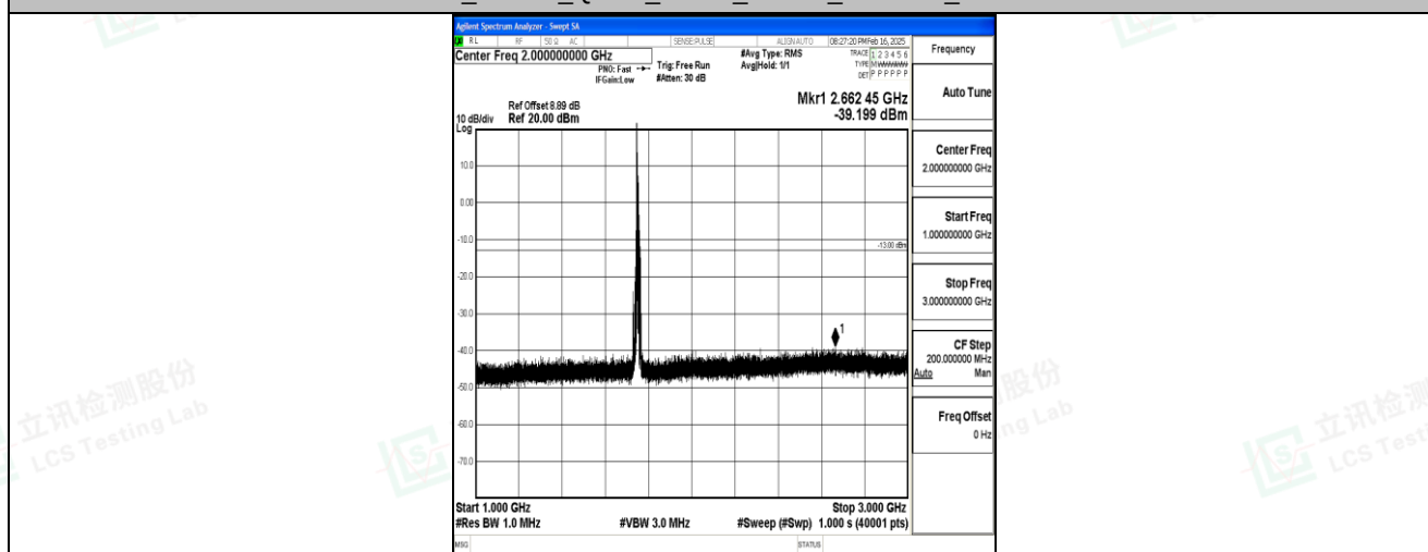
Band4_10MHz_QPSK_20350_1RB#0_1000~3000_1000~3000
