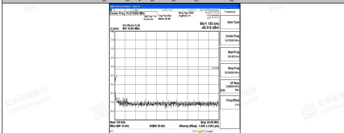
Band4_10MHz_16QAM_20350_1RB#0_0.15~30_0.15~30
