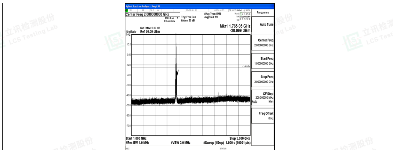
Band4_5MHz_16QAM_20375_1RB#0_1000~3000_1000~3000
