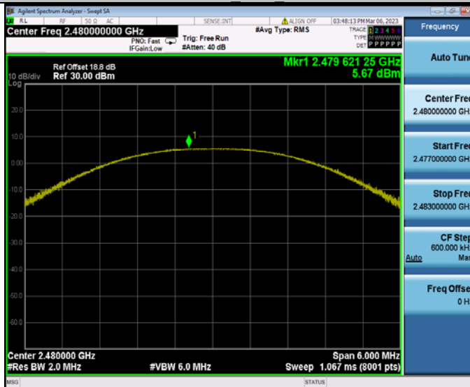
SRD2.4G Ant2 2480
