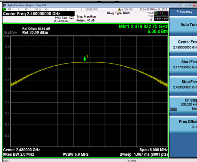
SRD2.4G Ant2 2480
