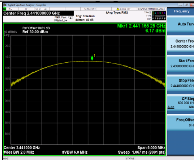
SRD2.4G Ant1_2441
