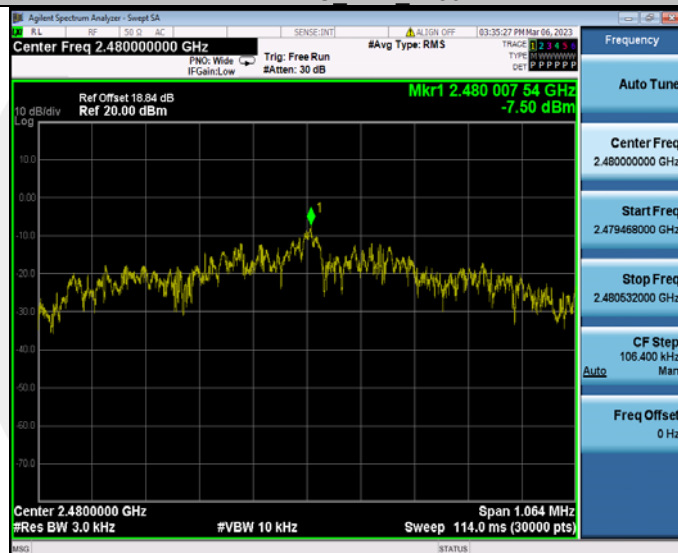
SRD2.4G Ant2 2480
