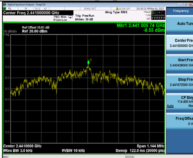
SRD2.4G Ant1_2441
