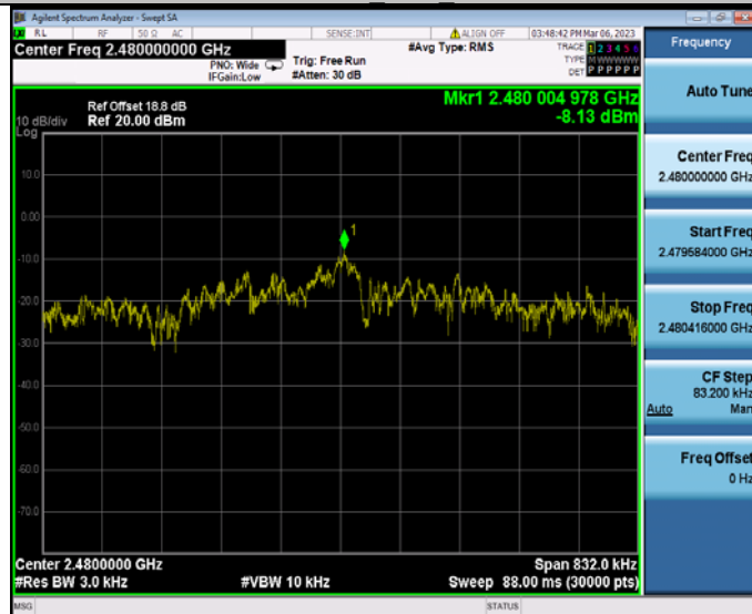
SRD2.4G Ant2 2480
