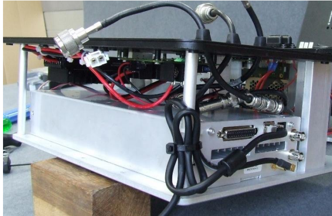
Photograph 05: Internal view – Left Side
