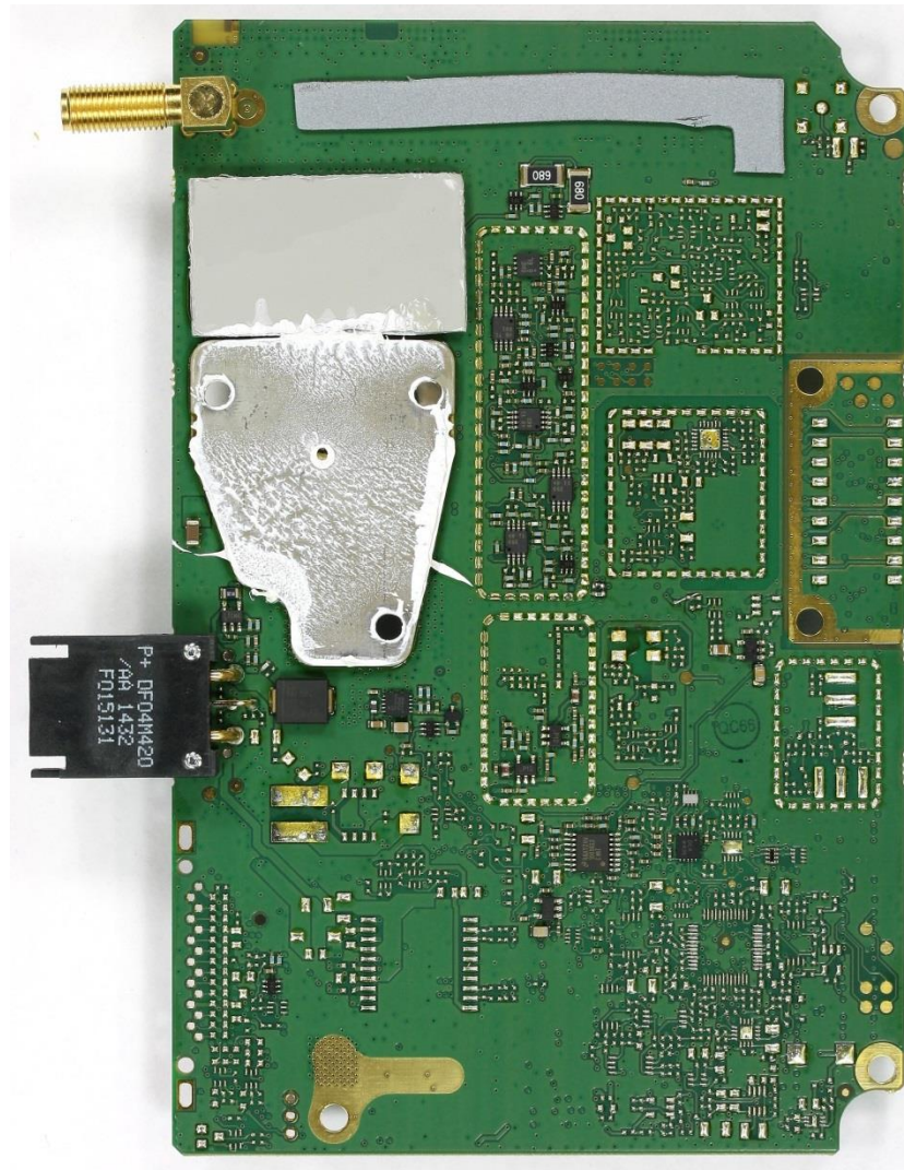
Photograph 13: Power Amplifier PCB – Bottom
