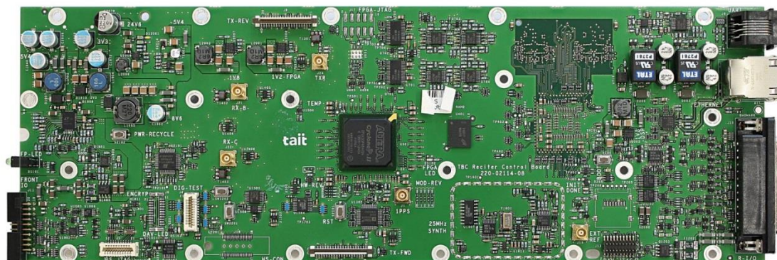
Photograph 15: Reciter Control Board (RCB) – Top (can off)
