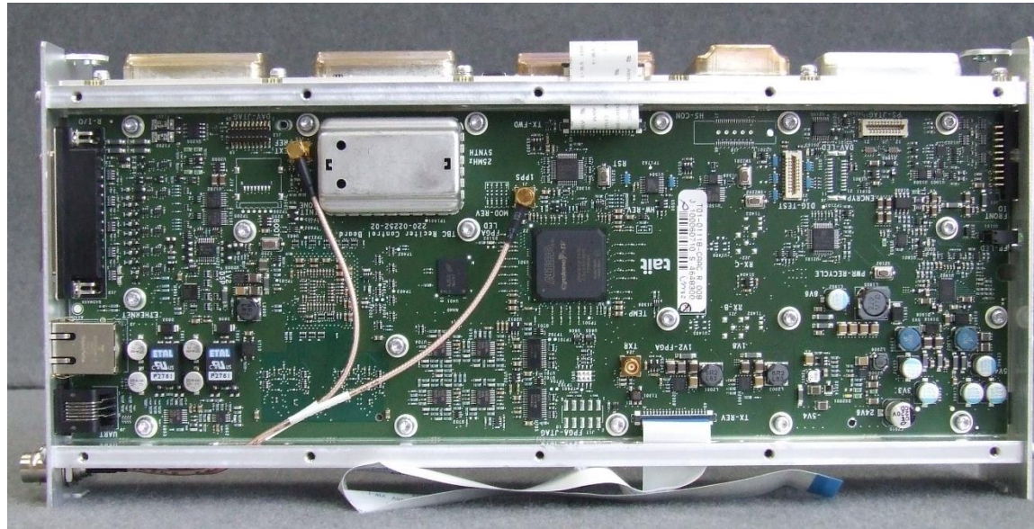
Photograph 14: Reciter Control Board (RCB) – Top
