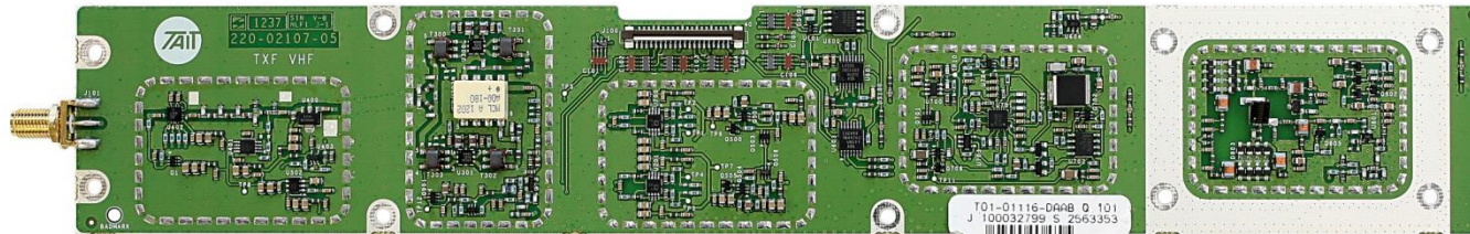
Photograph 21: Transmit Forward Power Board (TXF) – Top (cans off)
