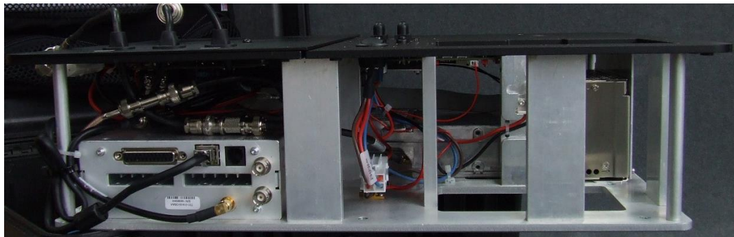
Photograph 03: Internal view – Front Side
