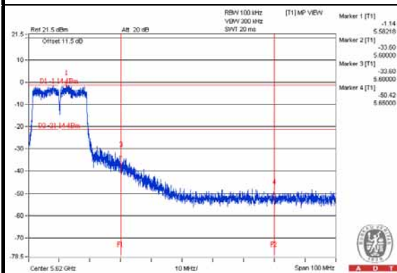
802.11ac (VHT20) MODULATION (CH 116: 5580MHz)
