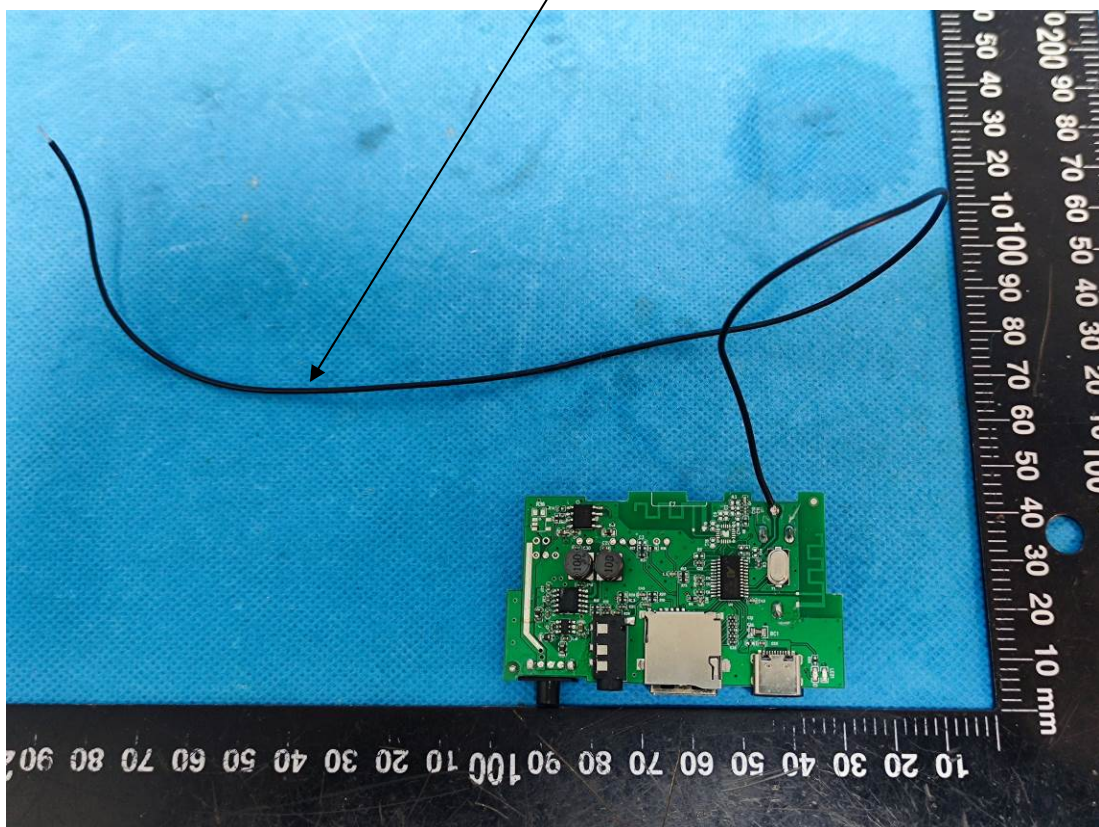
FM Antenna
