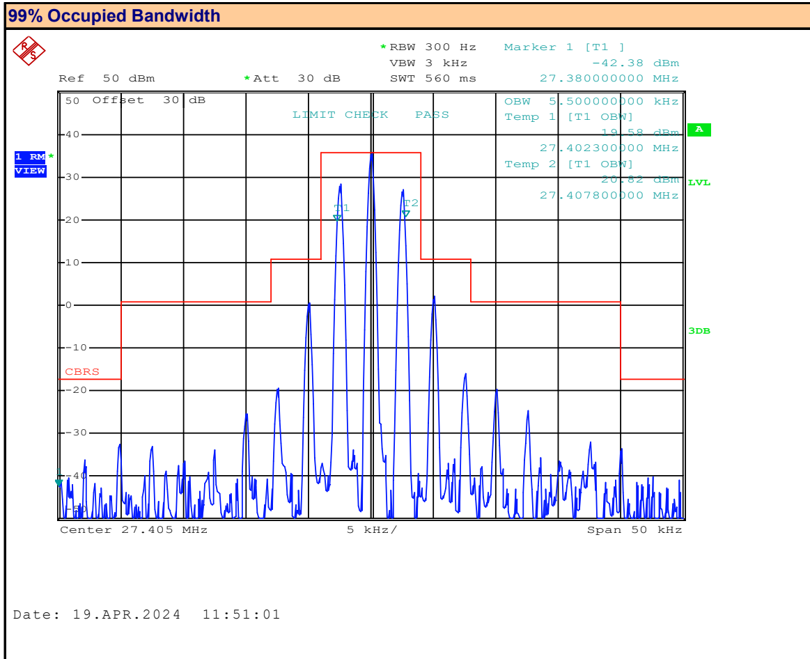
Plot 9.3 – Occupied Bandwidth, Channel 40, AM
