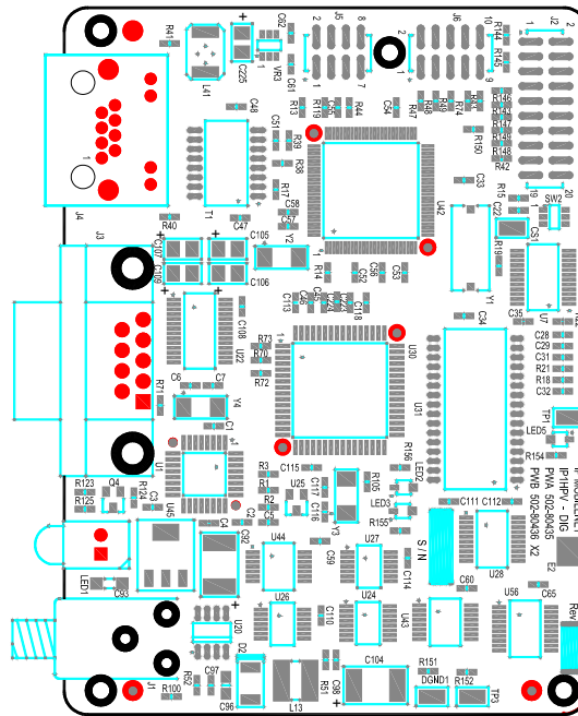
IPM4 Mobile Radio Digital Circuit Board
