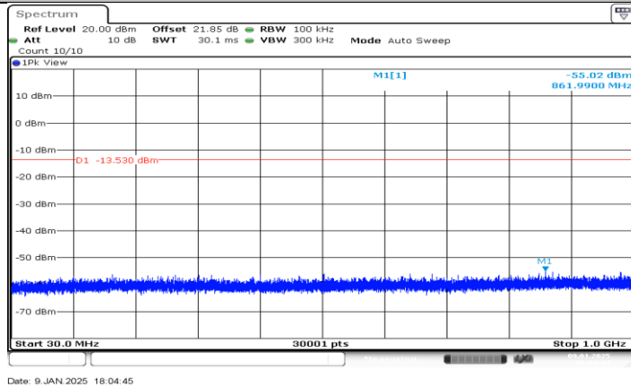
BLE_2M_Ant BT_2480_30~1000
