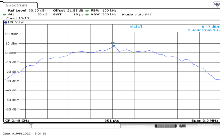
BLE_2M_Ant BT_2480_0~Reference
