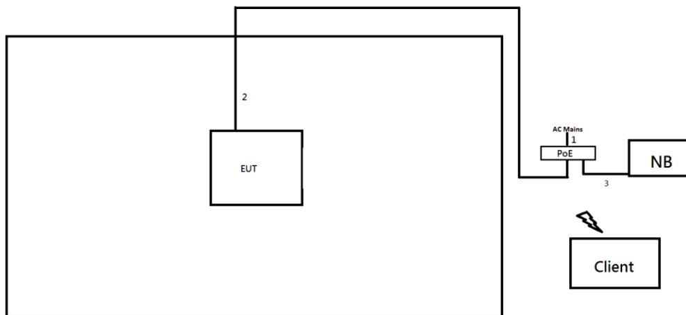
Test Setup Diagram - Radiated Test <Beamforming>
