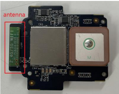
Figure 1.Antenna Actual Effect Picture
