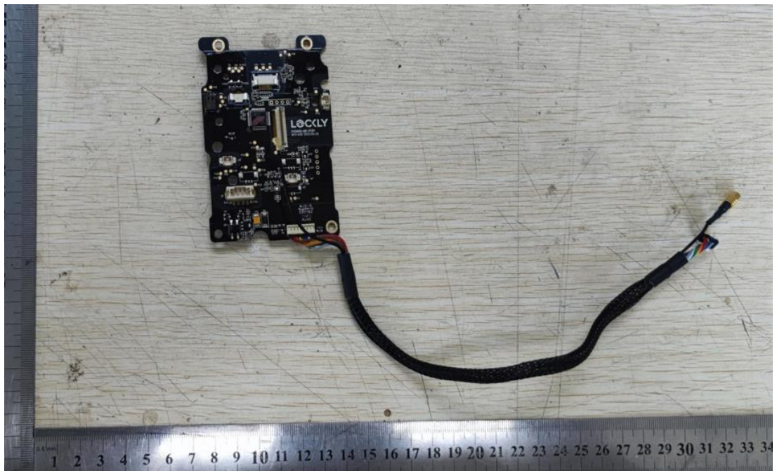
Inner Circuit Bottom View
