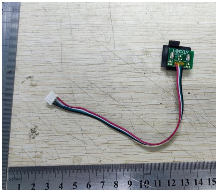
Inner Circuit Top View
