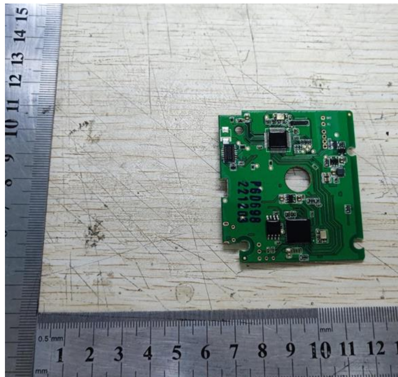
Inner Circuit Top View
