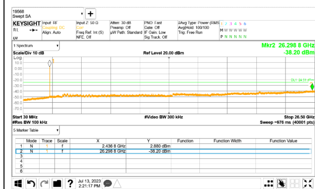
Out-Of-Band 6 Channel(4RU)
