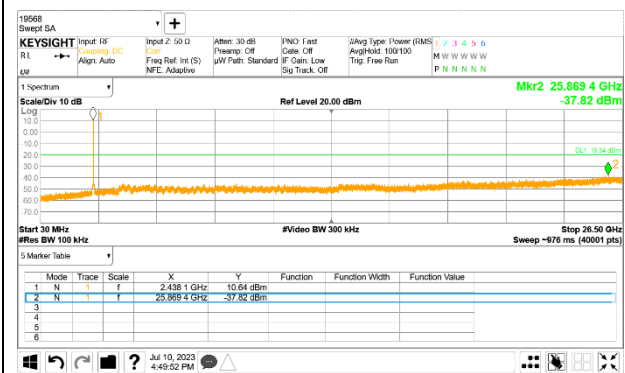
Out-Of-Band 6 Channel
