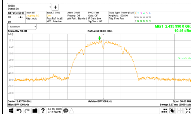
6 Channel Band-edge
