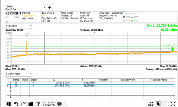
Out-Of-Band 11 Channel(4RU)
