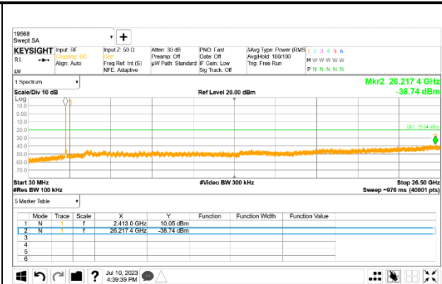
Out-Of-Band 1 Channel
