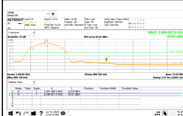
11 Channel Band-edge
