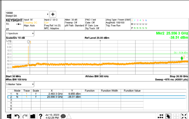
Out-Of-Band 11 Channel
