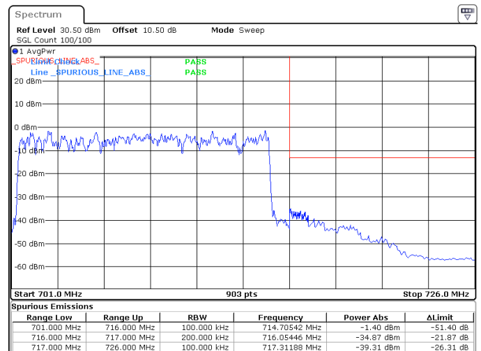
15MHz_15kHz_708.5MHz_DFT-s-OFDM QPSK_RB75@0 -34.87 dBm
