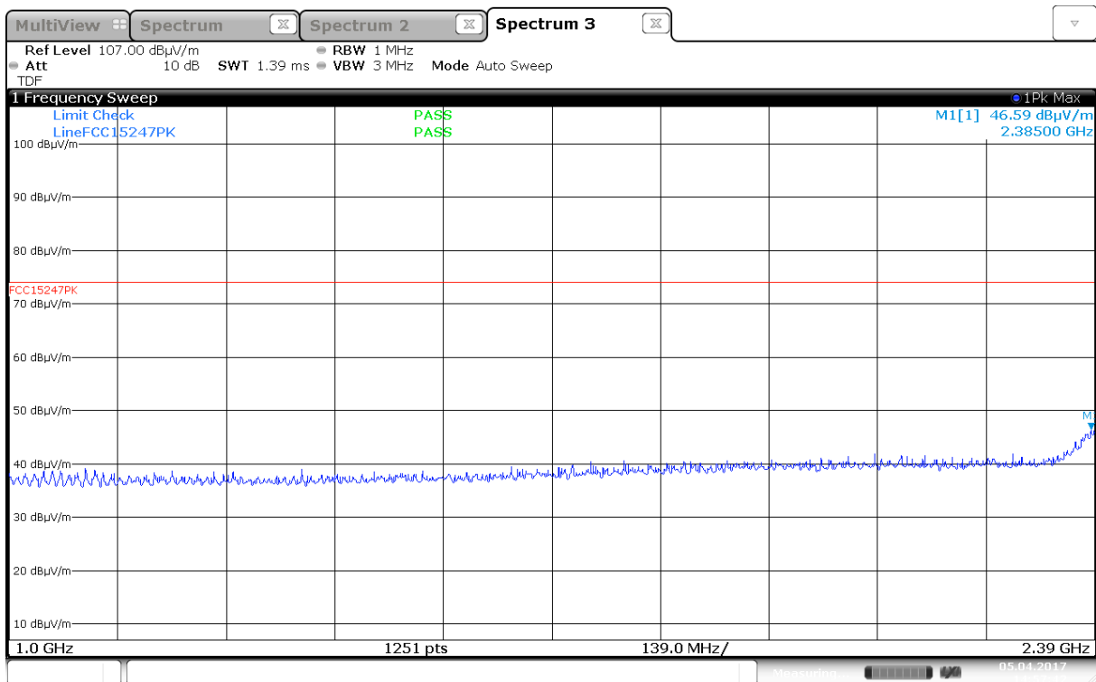
Radiated emissions, 1000 -2390MHz, VP, 2403MHz, EUT H2, Ant 1
