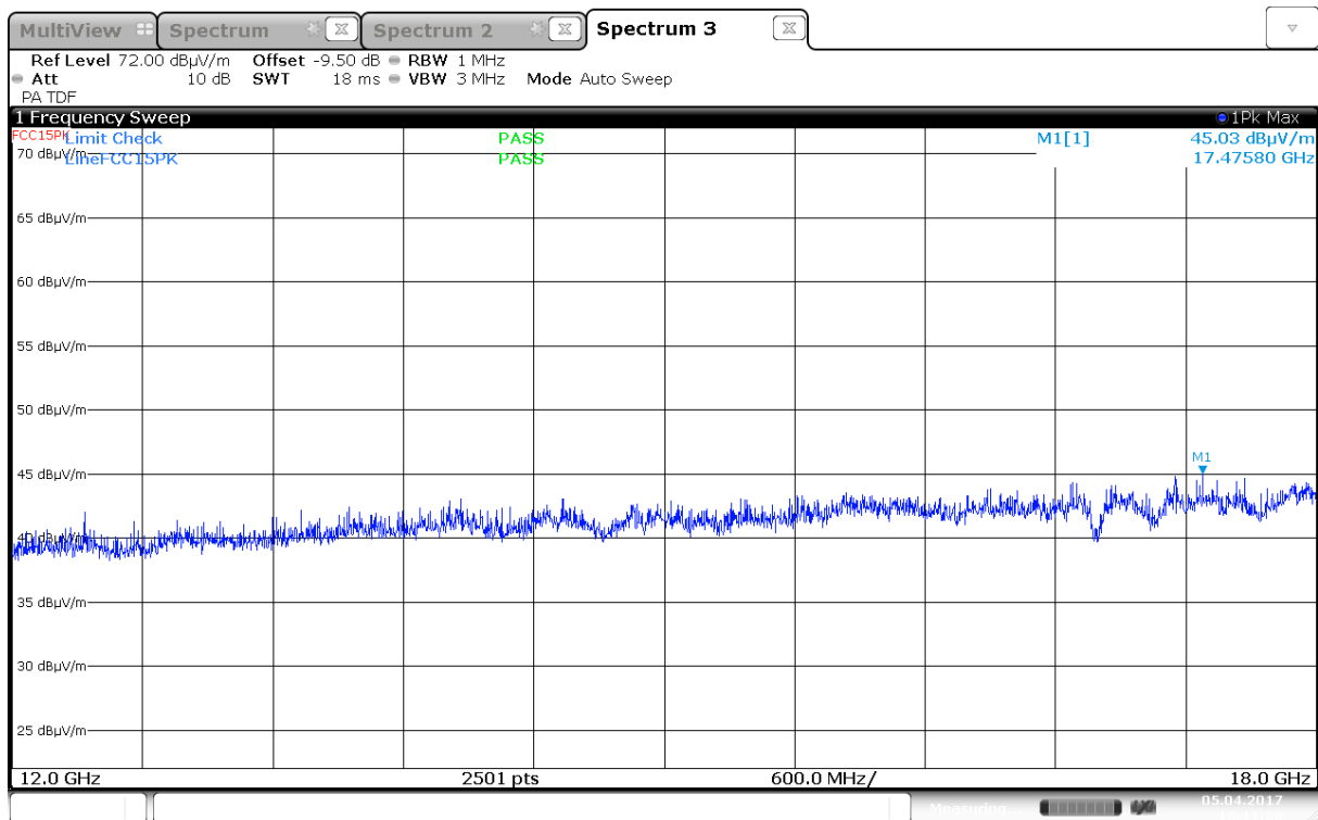
Radiated emissions, 12000 -18000MHz, HP, 2441MHz, EUT H2, Ant 1, @1m
