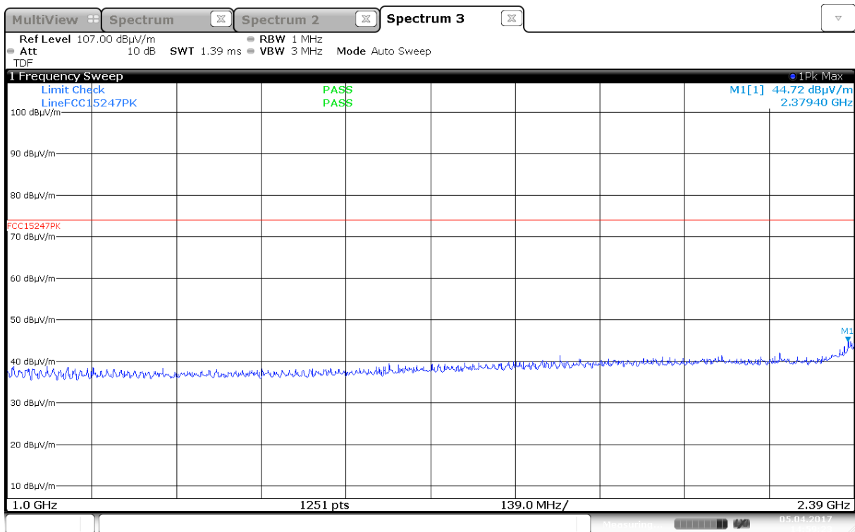
Radiated emissions, 1000 -2390MHz, HP, 2403MHz, EUT H2, Ant 1
