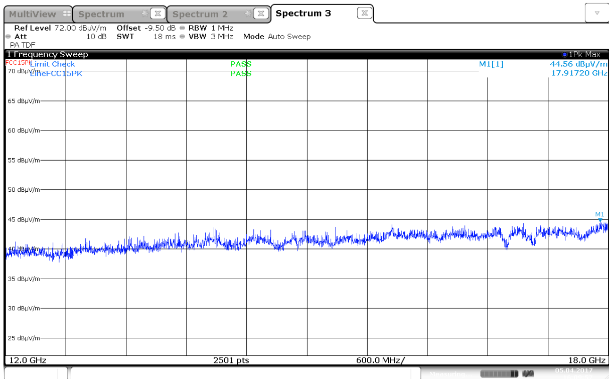
Radiated emissions, 12000 -18000MHz, VP, 2441MHz, EUT H2, Ant 1, @1m
