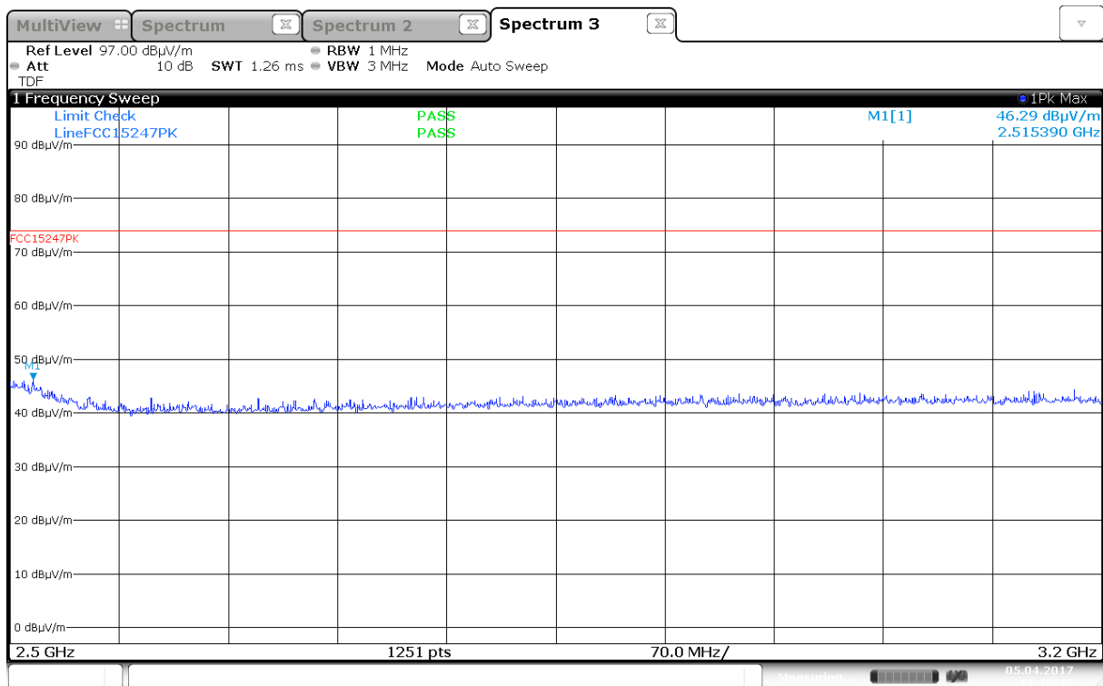
Radiated emissions, 2500 -3200MHz, VP, 2481MHz, EUT H2, Ant 1
