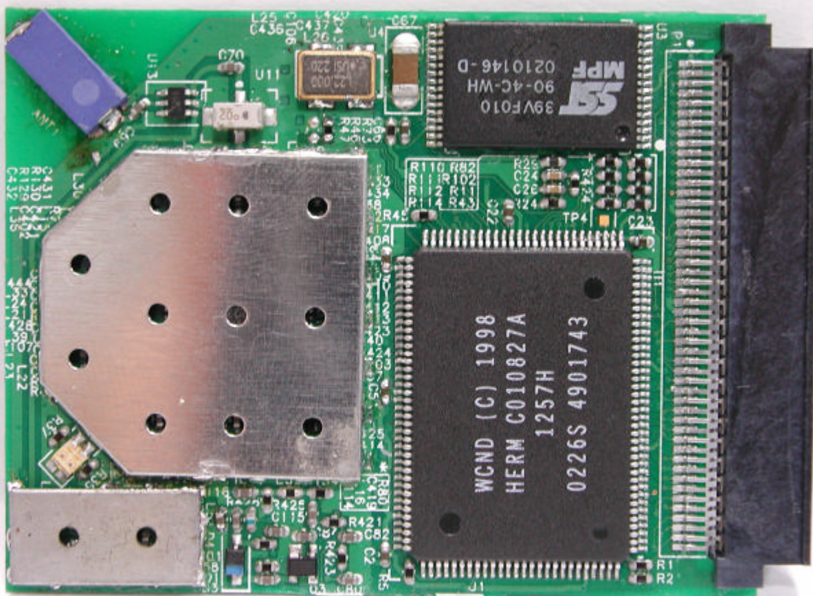
Internal Photo of USI 802.11b CompactFlash Card
