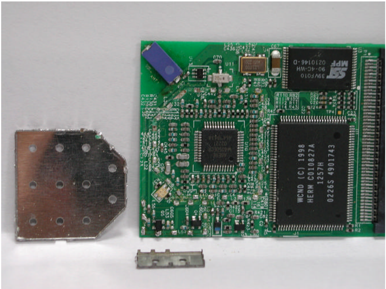
Internal Photo of USI 802.11b CompactFlash Card
