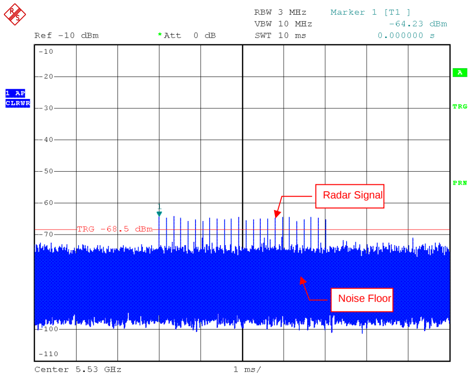
Radar Signal 2
