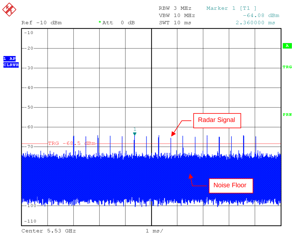
Radar Signal 3
