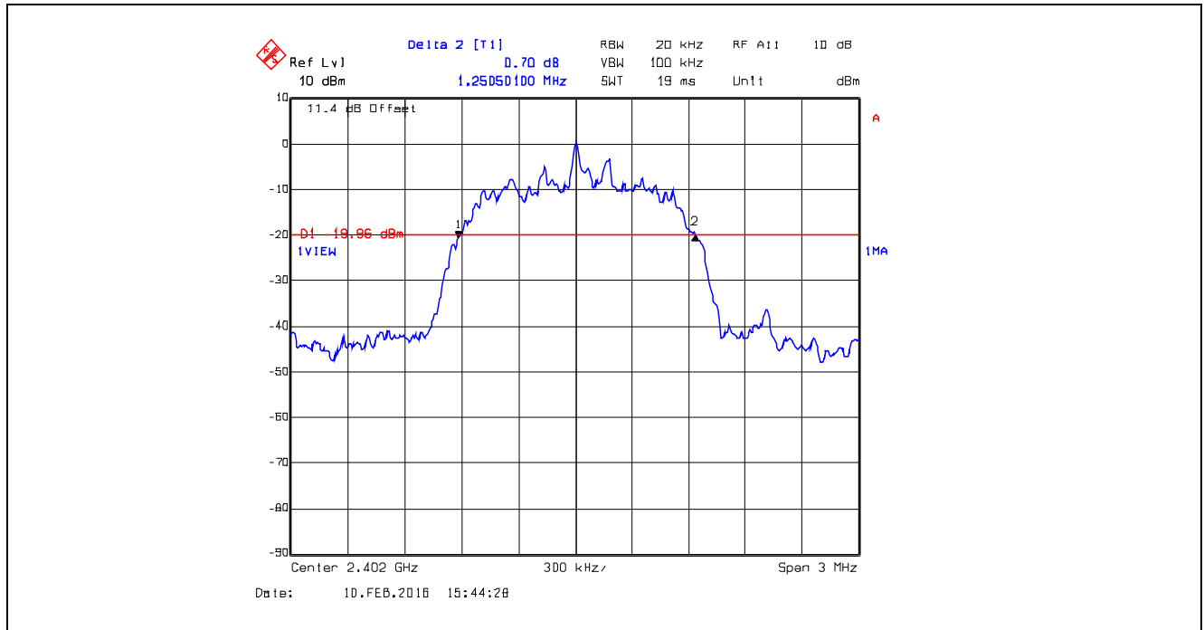
Plot 5.3.4.1.13. 20 dB Bandwidth, \pi/4 -DQPSK, 2DH3, CH 0, 2402 MHz
