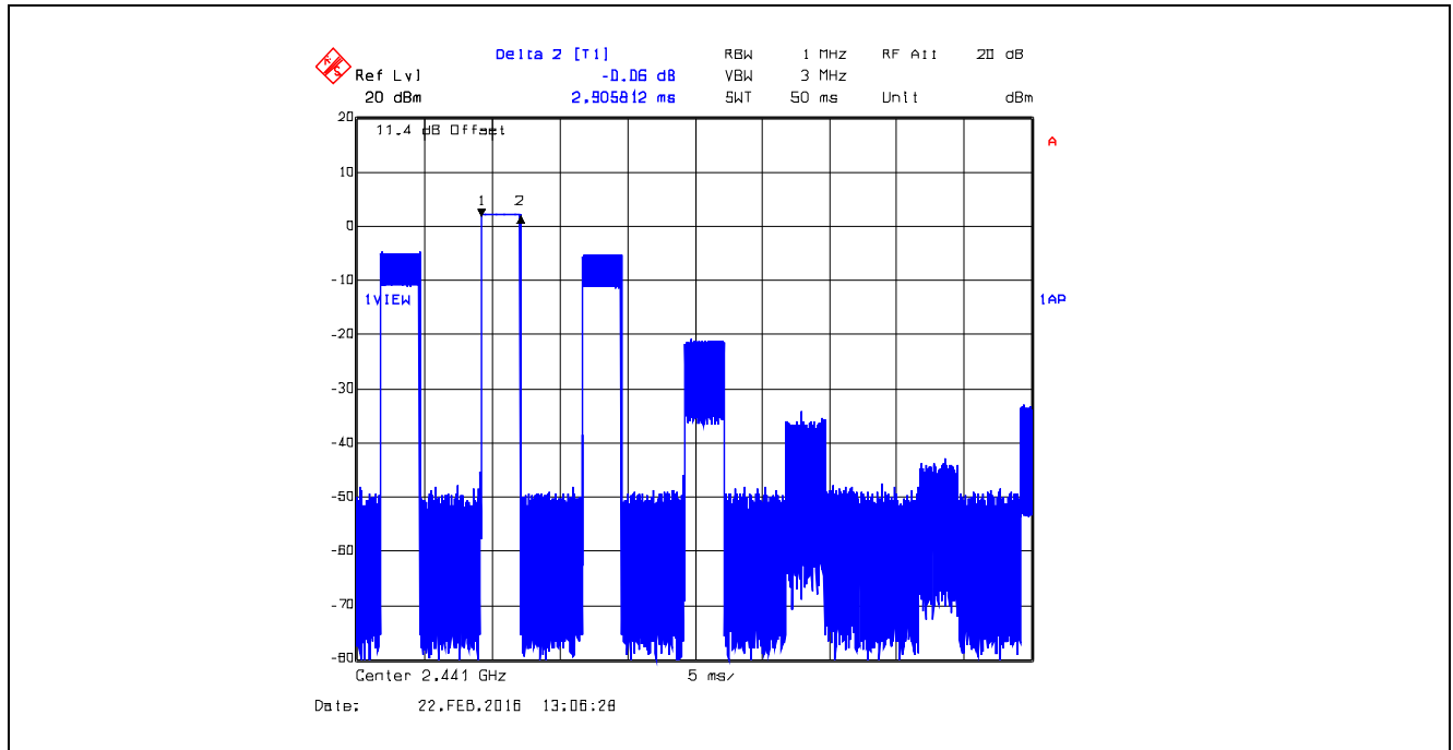
Plot 5.3.4.4.15. Time of Occupancy, GFSK, DH5, 2441 MHz Dwell Time @ 2441 MHz = 2.9058 ms
