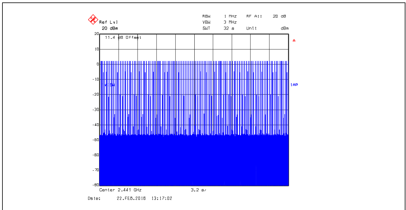
Plot 5.3.4.4.16. Time of Occupancy, GFSK, DH5, 2441 MHz Average time of occupancy = (Dwell Time) x (number of hops within a period) = 2.9058 ms x 107 = 310.92 ms
