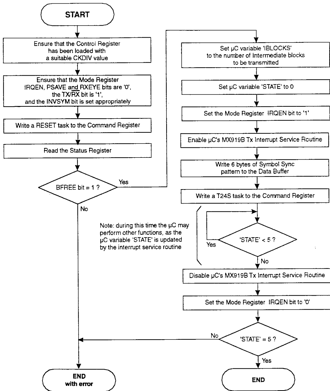
Figure 19: Transmit Frame Example Flowchart, Main Program
