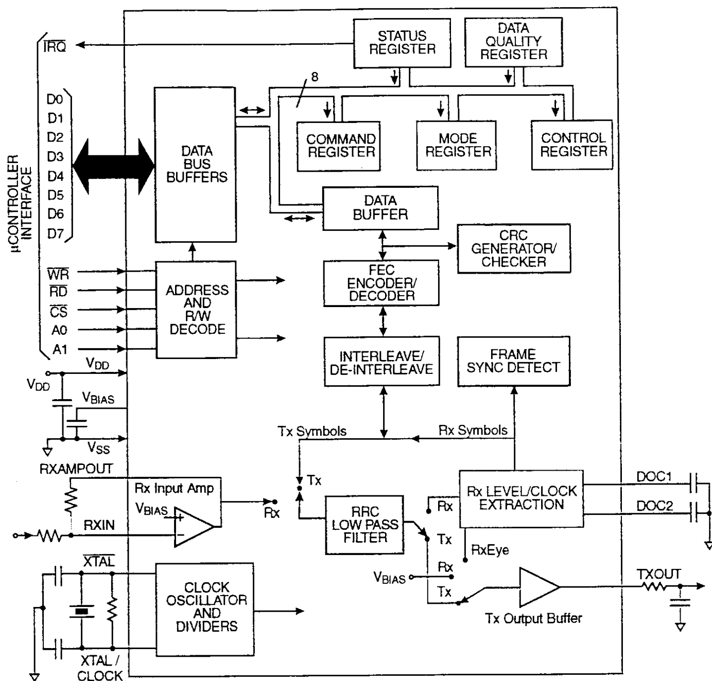
Figure 1: Block Diagram
