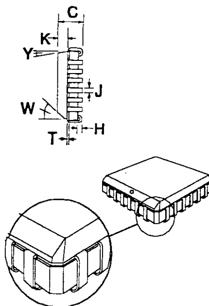
Figure 32: 24-pin PLCC Mechanical Outline : Order as part no. MX919BLH
