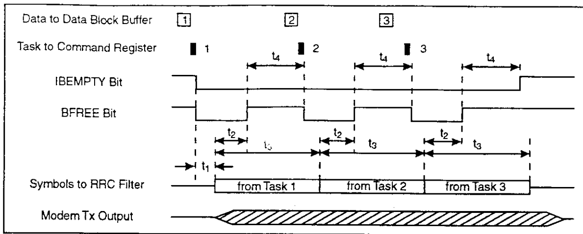
Figure 11: Transmit Task Timing Diagram
