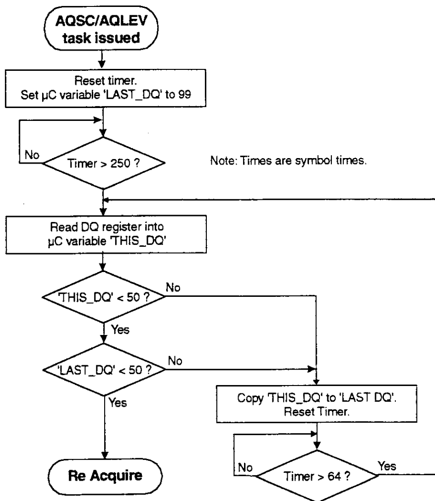
Figure 27: Received Signal Quality Monitor Flowchart
