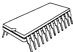
Figure 33: 24-pin PDIP Mechanical Outline: Order as part no. MX919BP
