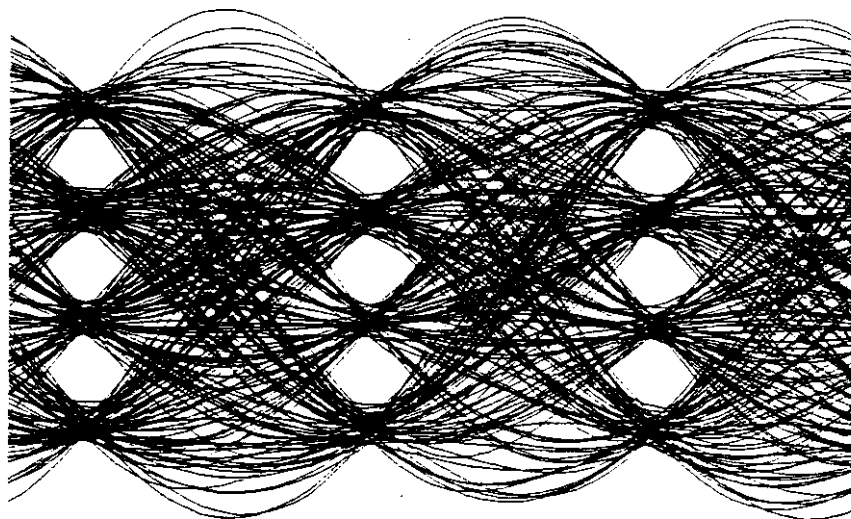
Figure 17: Tx Signal Eye TXIMP = 0
