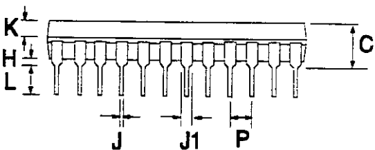
Figure 33: 24-pin PDIP Mechanical Outline: Order as part no. MX919BP
