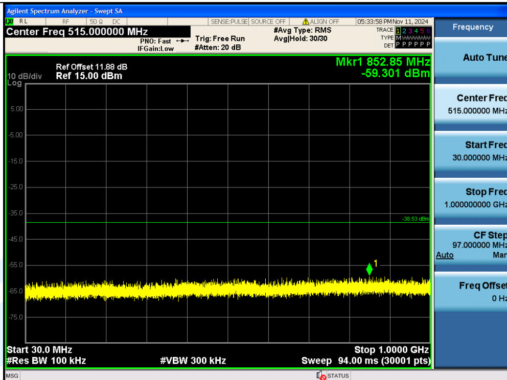
DH5-Ant1-2441-30~1000-PASS
