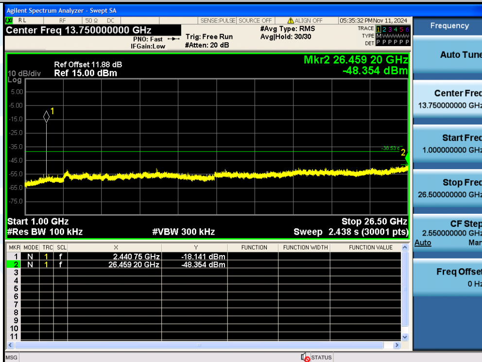
DH5-Ant1-2441-1000~26500-PASS
