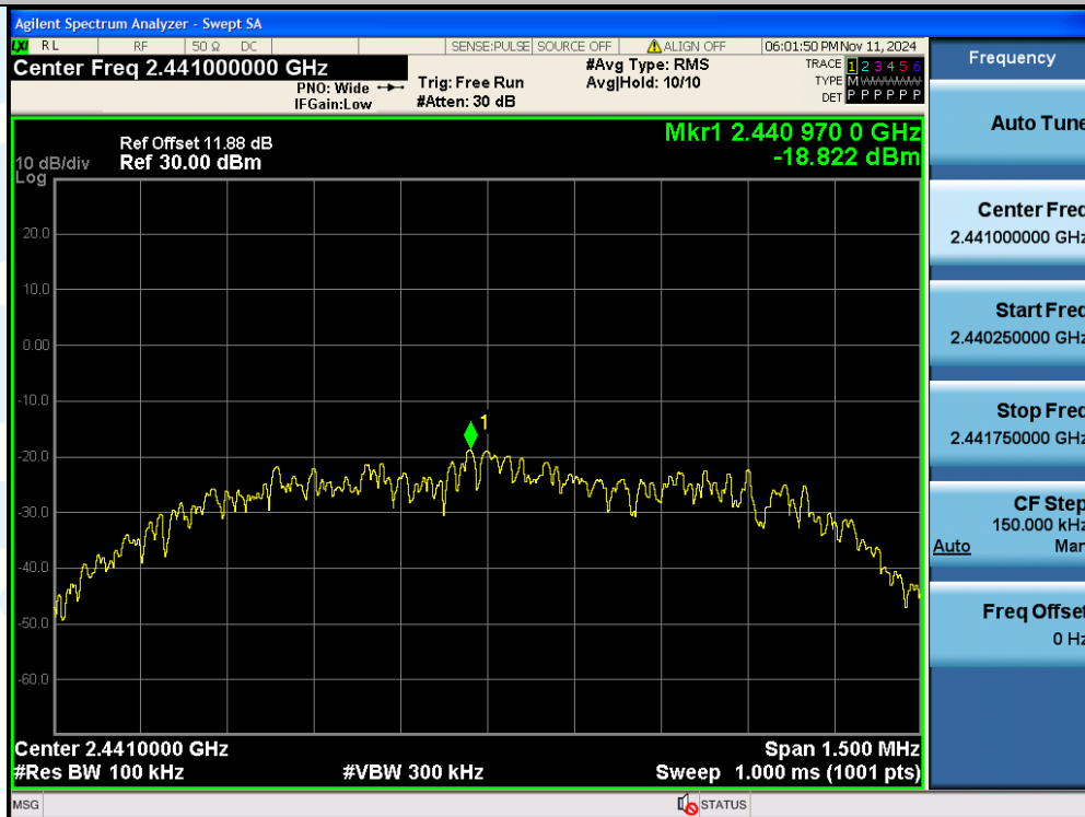
3DH5-Ant1-2441-0~Reference-PASS
