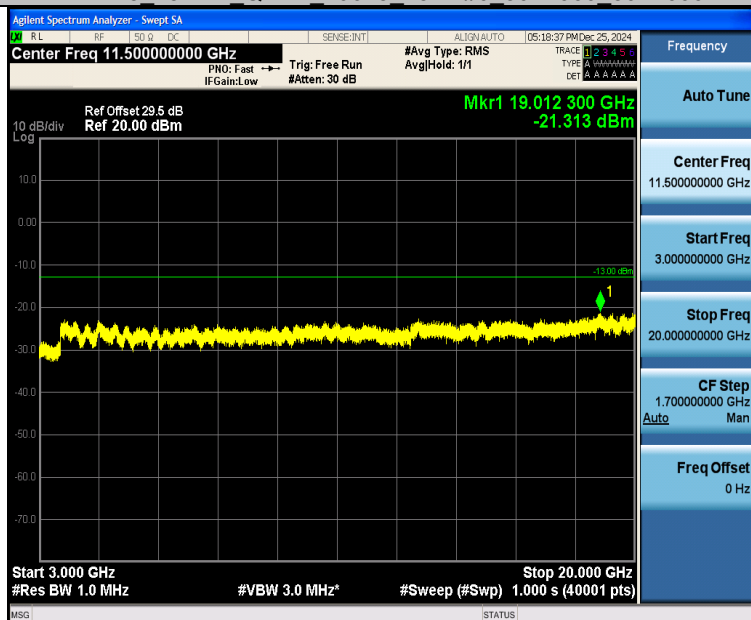
Band25_15MHz_QPSK_26615_75RB#0_3000~20000_3000~20000
