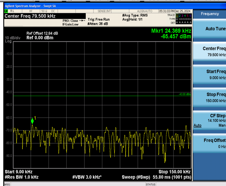
Band25_20MHz_QPSK_26140_1RB#0_0.009~0.15_0.009~0.15
