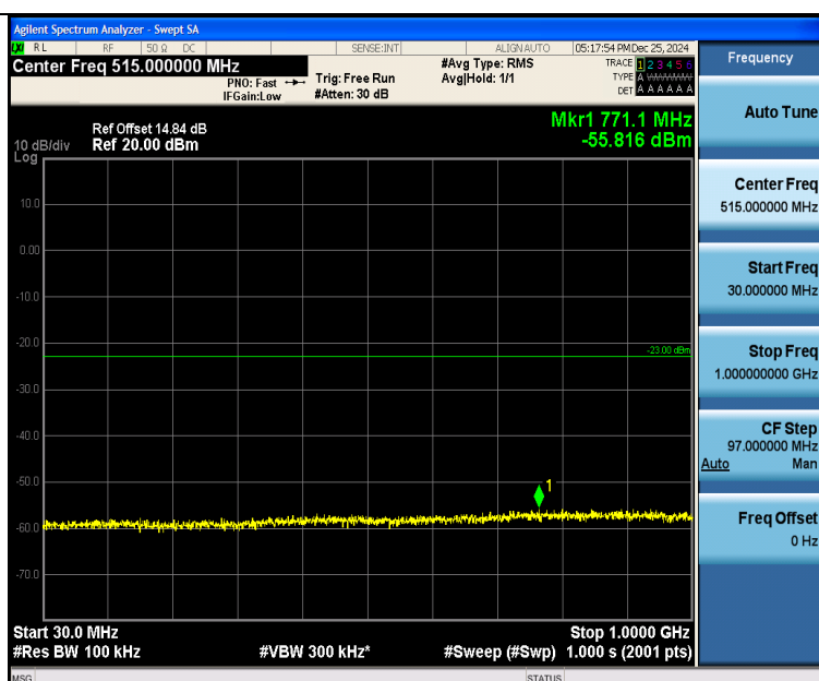
Band25_15MHz_QPSK_26615_75RB#0_30~1000_30~1000
