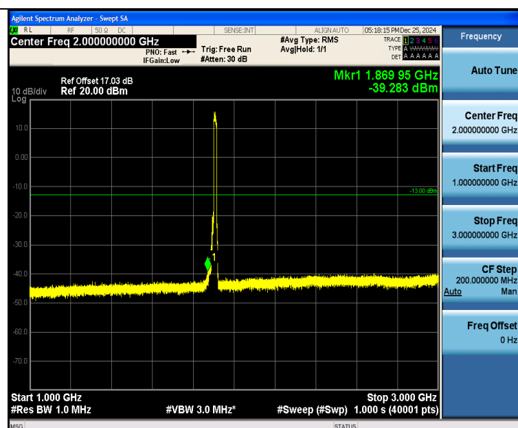
Band25_15MHz_QPSK_26615_75RB#0_1000~3000_1000~3000
