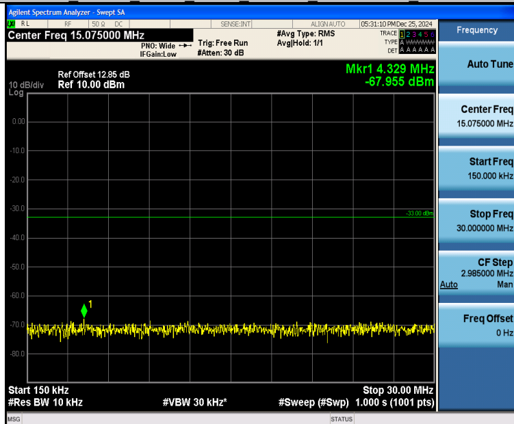
Band25_20MHz_QPSK_26140_1RB#0_0.15~30_0.15~30
