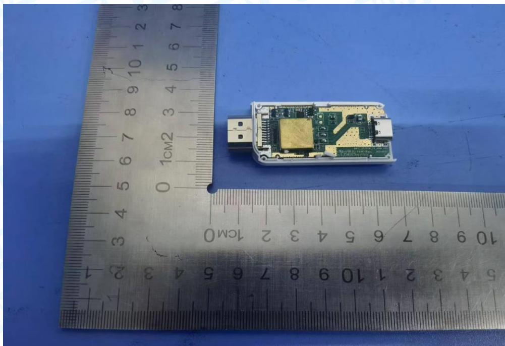
Photo 8 Internal of EUT
