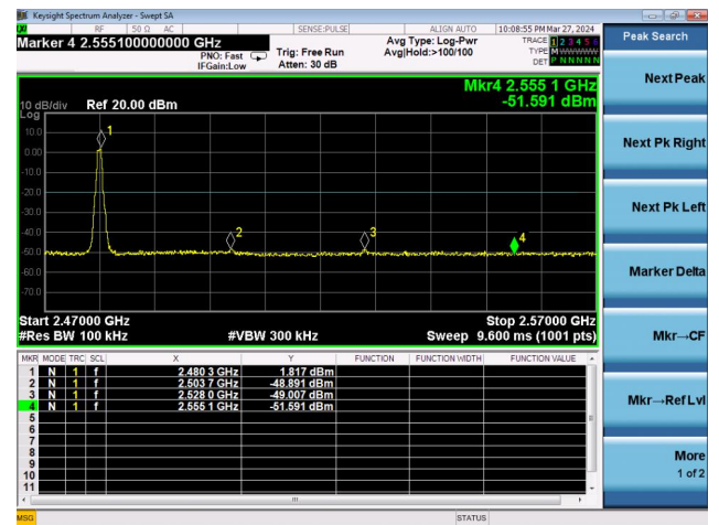
Right bandedge
