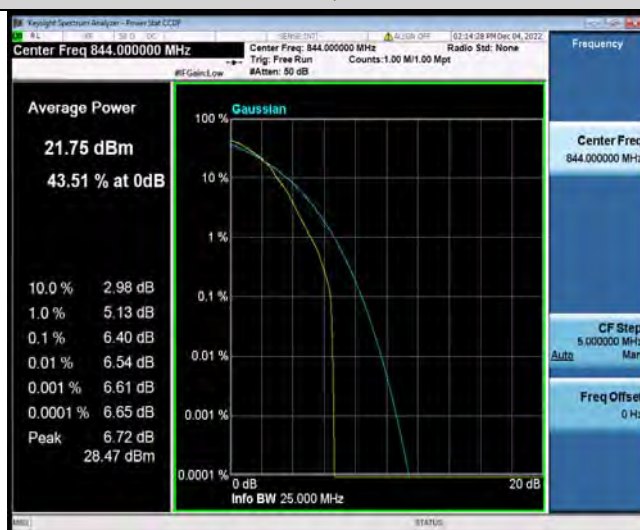
Band5-10MHz-64QAM-20600-50RB#0
