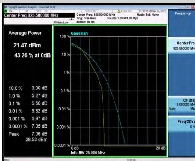
Band5-3MHz-64QAM-20415-15RB#0
