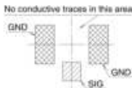
Figure 39: U.FL surface mounted connector mounting pattern layout
