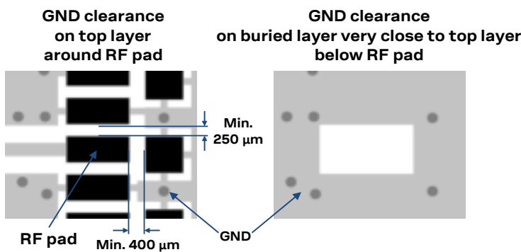
Figure 35: GND keep-out area on top layer around RF pad and on very close buried layer below RF pad (ANT / ANT_GNSS)
