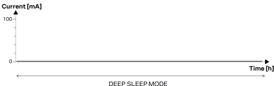
Figure 11: Example of VCC current consumption profile in ultra low power deep sleep mode with the use of the PSM enabled (AT+CPSMS≠0), module registered with the network: the module is in ultra low power deep sleep mode, with no concurrent activities executed, and it does not periodically wake up for paging block reception, but it wakes up upon the expiration of the periodic update timer set by the network or due to proper toggling of the PWR_ON / PWR_CTRL input line
