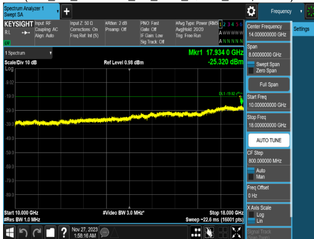
Plot 8-117. Conducted Spurious Emission Plot 10 GHz to 18 GHz (n70_1C_25M+n66_1C_15M_QPSK_Low, Port 0)
