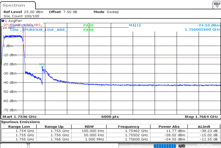
1.4MHz_High_QPSK_6@0 -24.55 dBm
