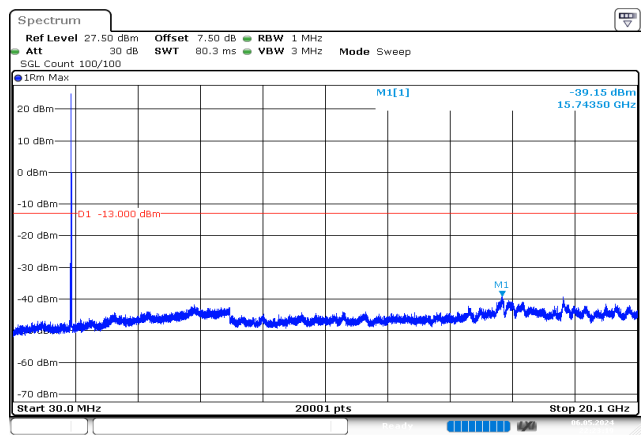
15MHz_High_QPSK_1@0 -39.15 dBm
