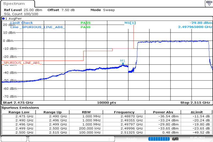
15MHz_Low_QPSK_75@0 -29.80 dBm
