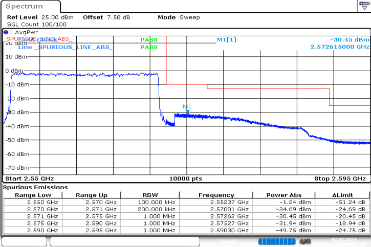
20MHz_High_QPSK_100@0 -30.45 dBm
