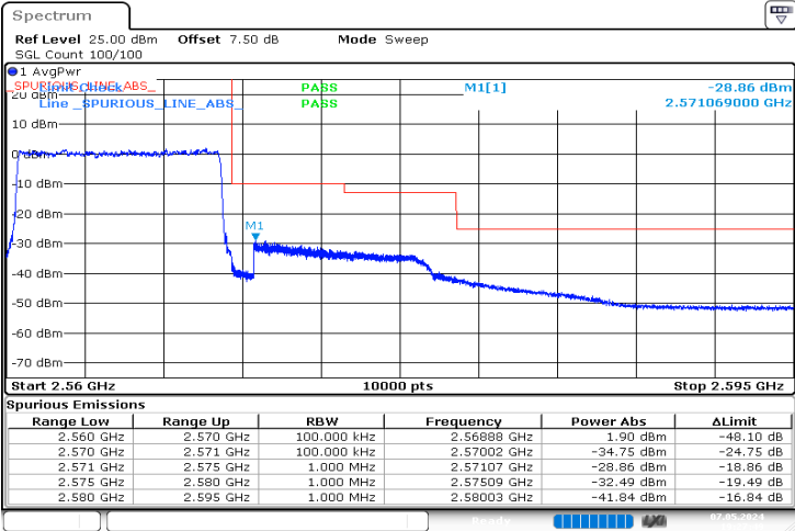
10MHz_High_QPSK_50@0 -28.86 dBm
