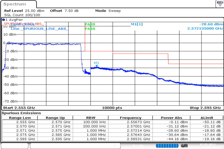
15MHz_High_QPSK_75@0 -28.60 dBm
