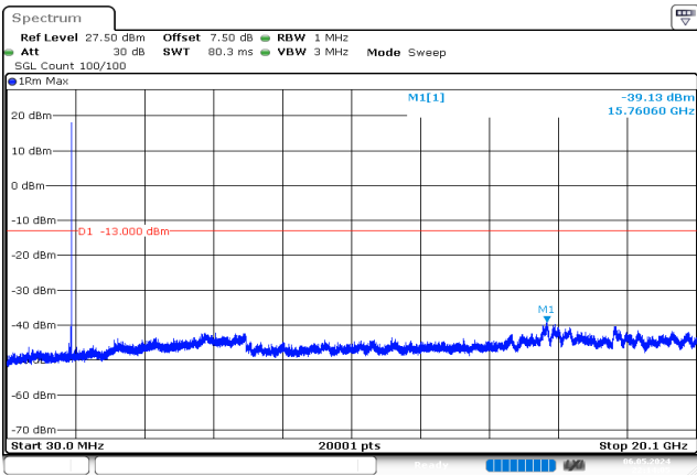
5MHz_High_QPSK_25@0 -39.13 dBm
