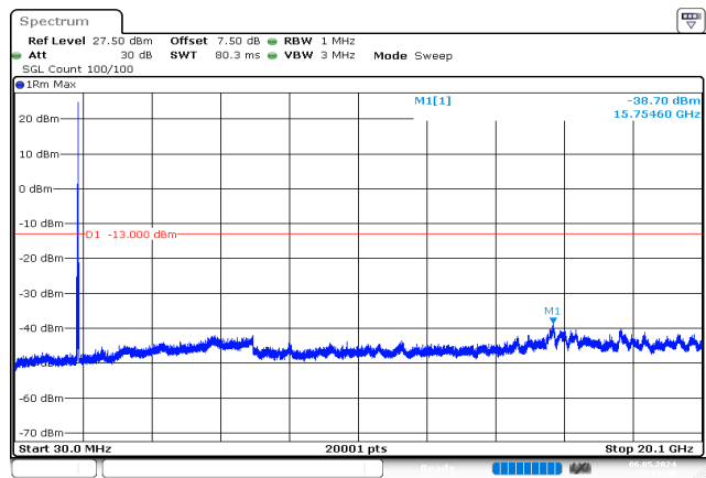
15MHz_Middle_QPSK_1@0 -38.70 dBm
