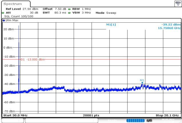
20MHz_Middle_QPSK_1@0 -39.52 dBm
