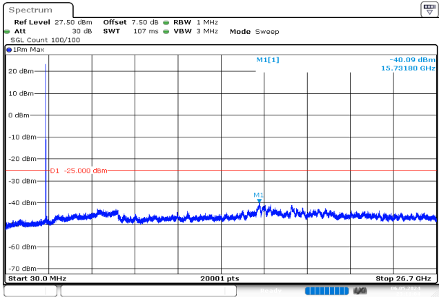
15MHz_Low_QPSK_1@0 -40.09 dBm
