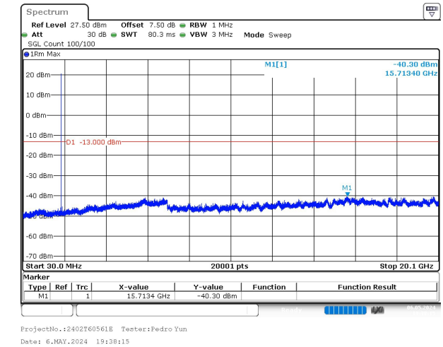
1.4MHz_Low_QPSK_1@0 -40.30 dBm
