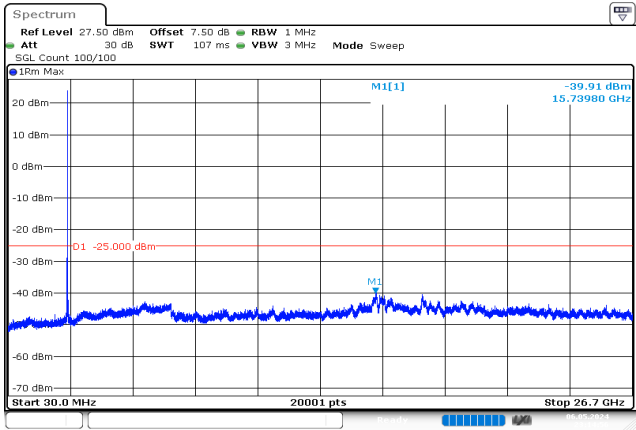
15MHz_High_QPSK_1@0 -39.91 dBm
