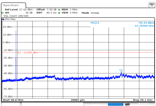
15MHz_Low_QPSK_75@0 -39.43 dBm
