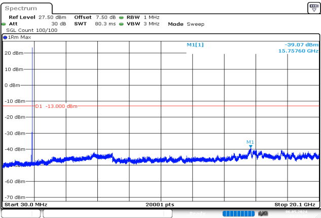
5MHz_High_QPSK_1@0 -39.07 dBm
