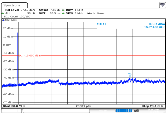
15MHz_High_QPSK_75@0 -39.04 dBm
