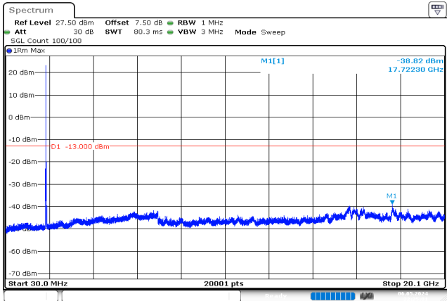
20MHz_Low_QPSK_1@0 -38.82 dBm
