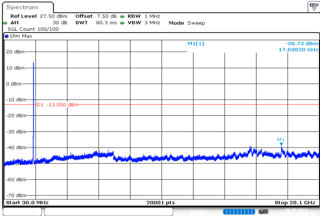
20MHz_High_QPSK_100@0 -38.73 dBm
