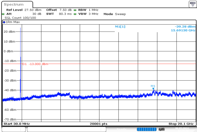
20MHz_High_QPSK_1@0 -39.28 dBm
