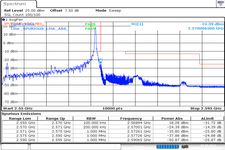
20MHz_High_QPSK_1@99 -24.39 dBm
