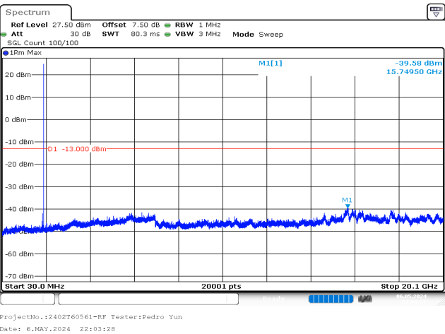
1.4MHz_High_QPSK_1@0 -39.58 dBm
