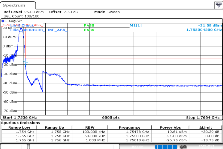
1.4MHz_High_QPSK_1@5 -21.08 dBm
