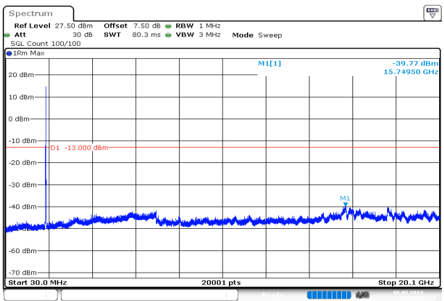
15MHz_Middle_QPSK_75@0 -39.77 dBm
