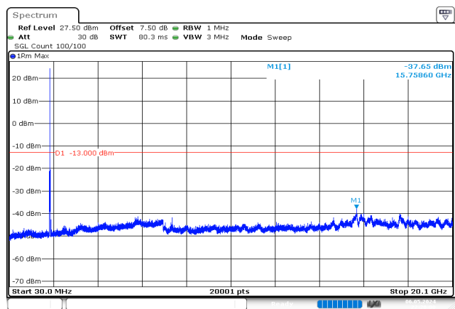
15MHz_Low_QPSK_1@0 -37.65 dBm
