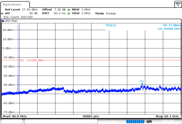
5MHz_Middle_QPSK_1@0 -39.72 dBm
