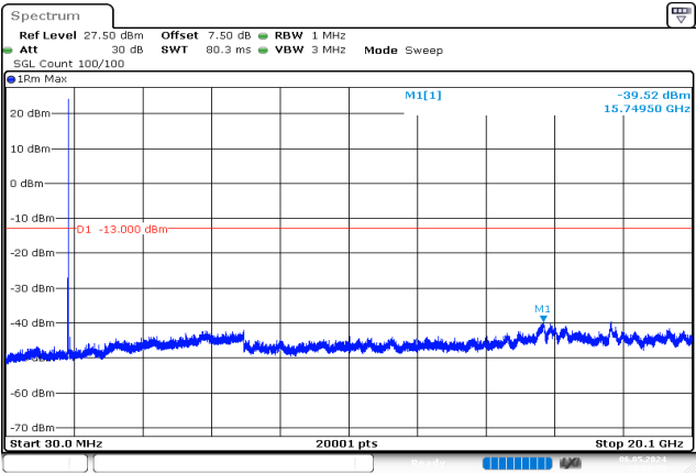
5MHz_Low_QPSK_1@0 -39.52 dBm
