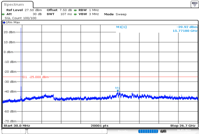
15MHz_Middle_QPSK_1@0 -39.92 dBm
